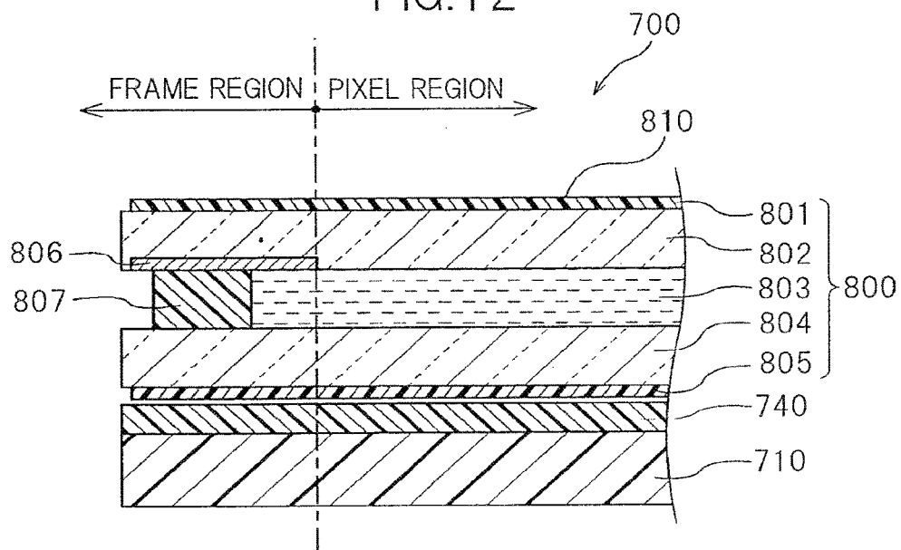
FIG. 12 (Prior Art)
