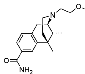
Compound 14
