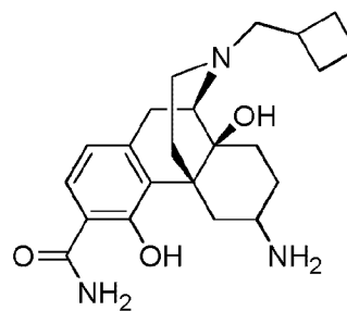
Compound 10
