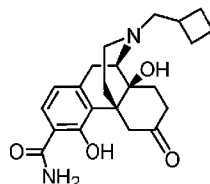
Compound A
