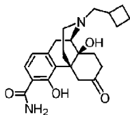
Compound A
