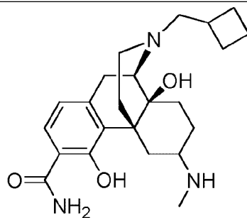
Compound 13
