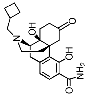
Compound A
