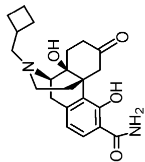
Compound A
