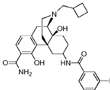
Compound 11
