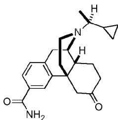
Compound 9
