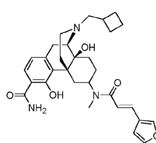
Compound 12
