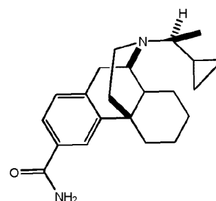
Compound 16
