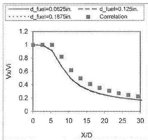
(a) Effect of fuel injection diameter
