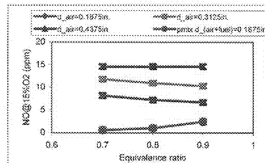
(b) NO emissions
