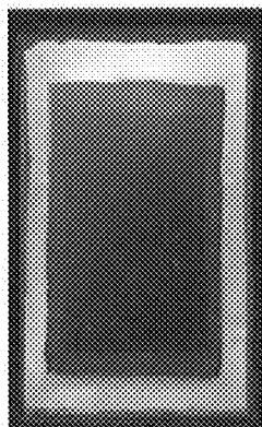
(b) \Phi=0.8 (premixed, d_{\text{air+fuel}}=0.1875\text{in.}
