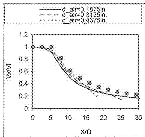
(b) Effect of air injection diameter
