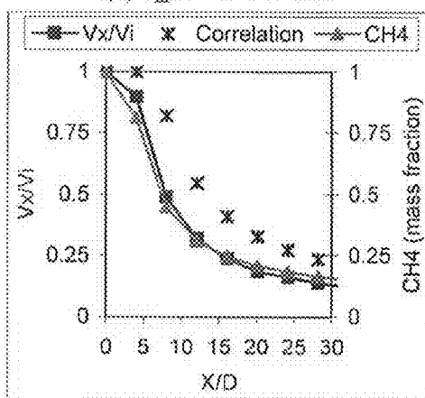
(e) d_{\text{air}}=0.4375 inch
