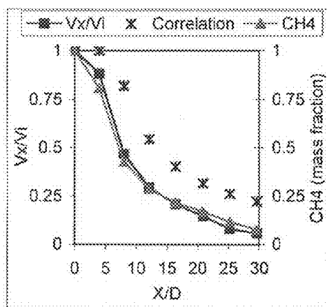
(a) d_{\text{fuel}}=0.0625 inch, d_{\text{air}}=0.1875 inch
