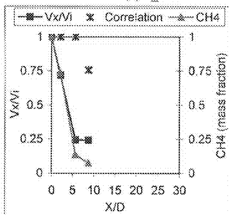
(b) d_{\text{fuel}}=0.125 inch
