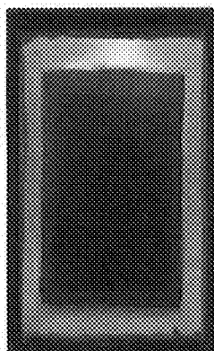
(a) \Phi=0.7 (premixed, d_{\text{air+fuel}}=0.1875\text{in.}
