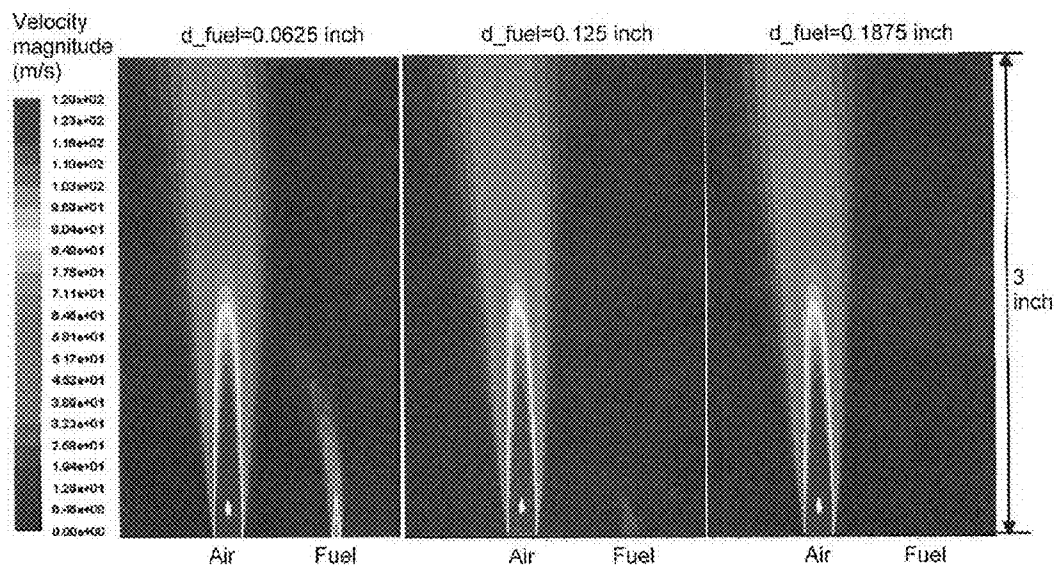
(a) Effect of fuel injection diameter ( d_{\text{air}}=0.1875 inch)
