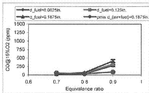
(a) CO emissions
