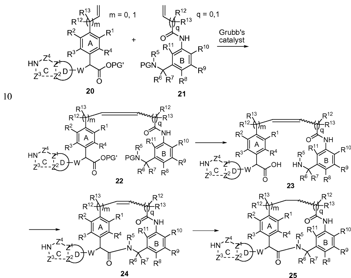
Scheme 5
