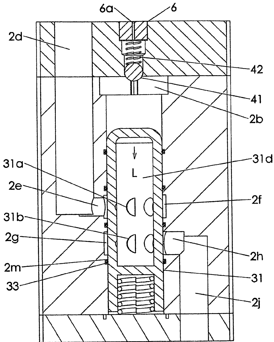
SECTION 102-102
