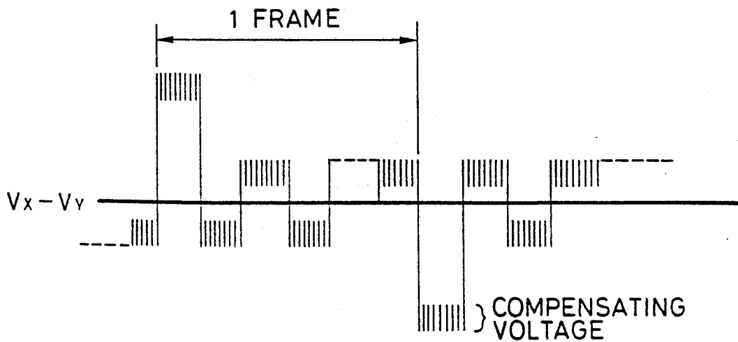
FIG. 1B VOLTAGE APPLIED TO PIXEL
