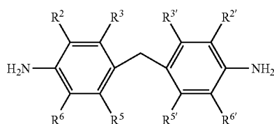
The 4,4'-methylenebis(aniline) backbone
