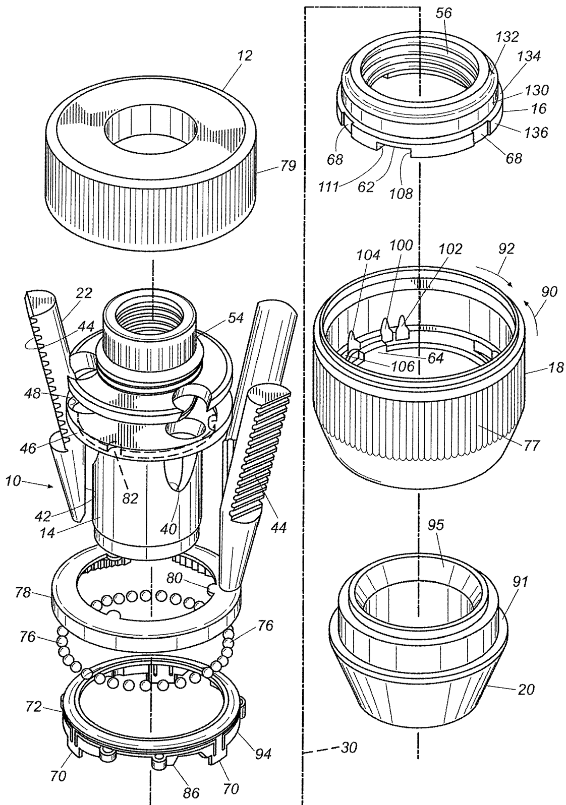
Fig. 2 (Prior Art)
