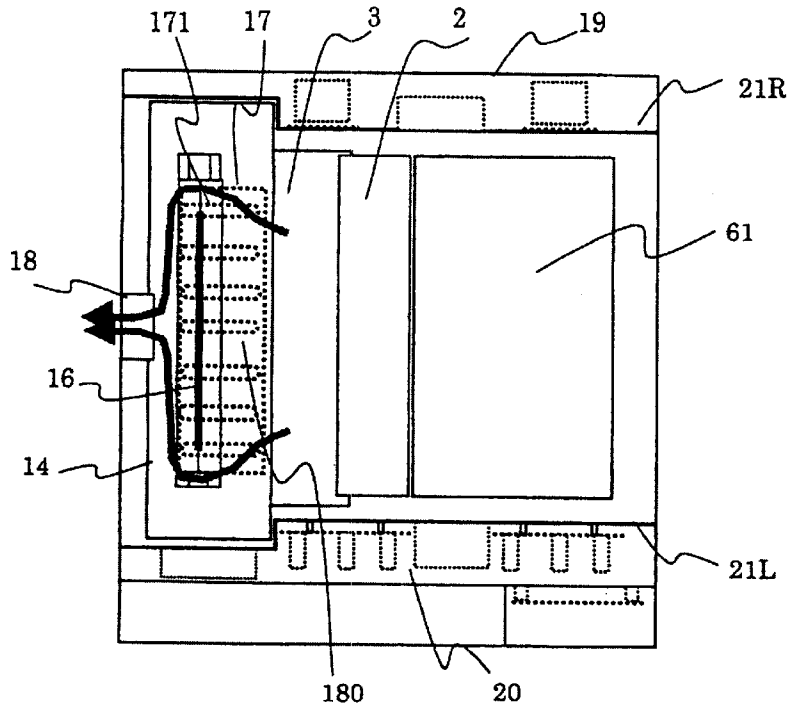
FIG. 3 PRIOR ART
