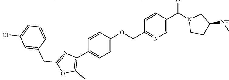
35 (3S)-1-([6-([4-[2-[(3-chlorophenyl)methyl]-5-methyl-1,3-oxazol-4-yl]phenoxy)methyl]pyridine-3-carbonyl]-N-methylpyrrolidin-3-amine
