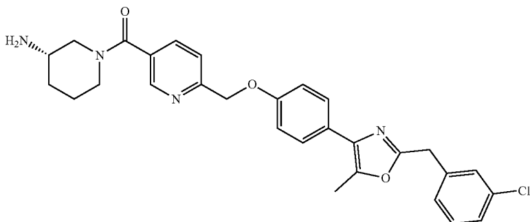
34 (3S)-1-([6-([4-[2-[(3-chlorophenyl)methyl]-5-methyl-1,3-oxazol-4-yl]phenoxy)methyl]pyridine-3-carbonyl]piperidin-3-amine
