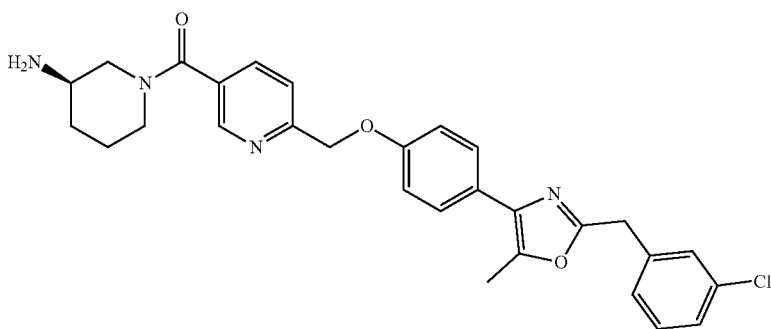
37 (3R)-1-([6-([4-[2-[(3-chlorophenyl)methyl]-5-methyl-1,3-oxazol-4-yl]phenoxy)methyl]pyridine-3-carbonyl]piperidin-3-amine
