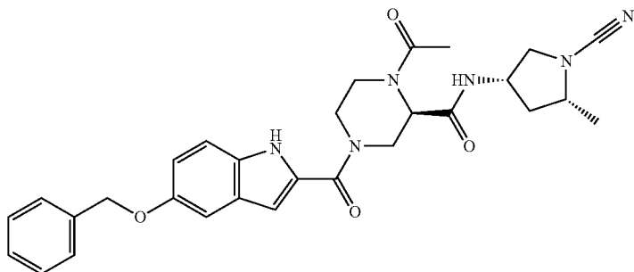
42 (2R)-1-Acetyl-4-[5-(benzyloxy)-1H-indole-2-carbonyl]-N-[(3S,5R)-1-cyano-5-methylpyrrolidin-3-yl]piperazine-2-carboxamide
