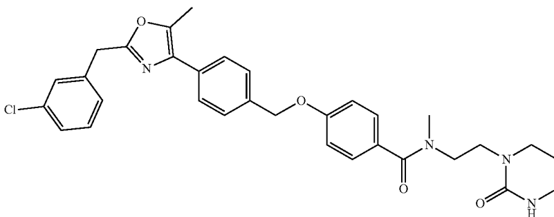
44 4-[(4-{2-[(3-Chlorophenyl)methyl]-5-methyl-1,3-oxazol-4-yl}phenyl)methoxy]-N-methyl-N-[2-(2-oxo-1,3-diazinan-1-yl)ethyl]benzamide
