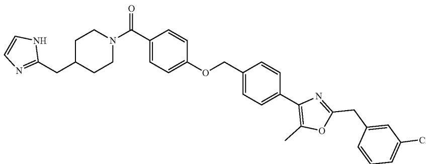
43 1-{4-[(4-{2-[(3-Chlorophenyl)methyl]-5-methyl-1,3-oxazol-4-yl}phenyl)methoxy]benzoyl}-4-[(1H-imidazol-2-yl)methyl]piperidine
