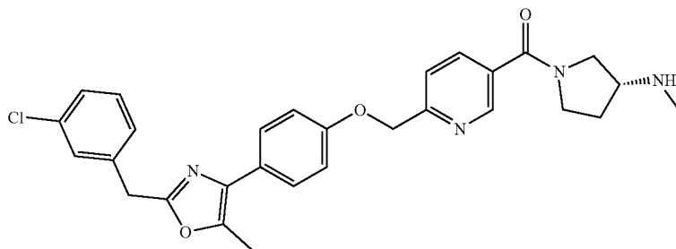
36 (3R)-1-([6-([4-[2-[(3-chlorophenyl)methyl]-5-methyl-1,3-oxazol-4-yl]phenoxy)methyl]pyridine-3-carbonyl]-N-methylpyrrolidin-3-amine
