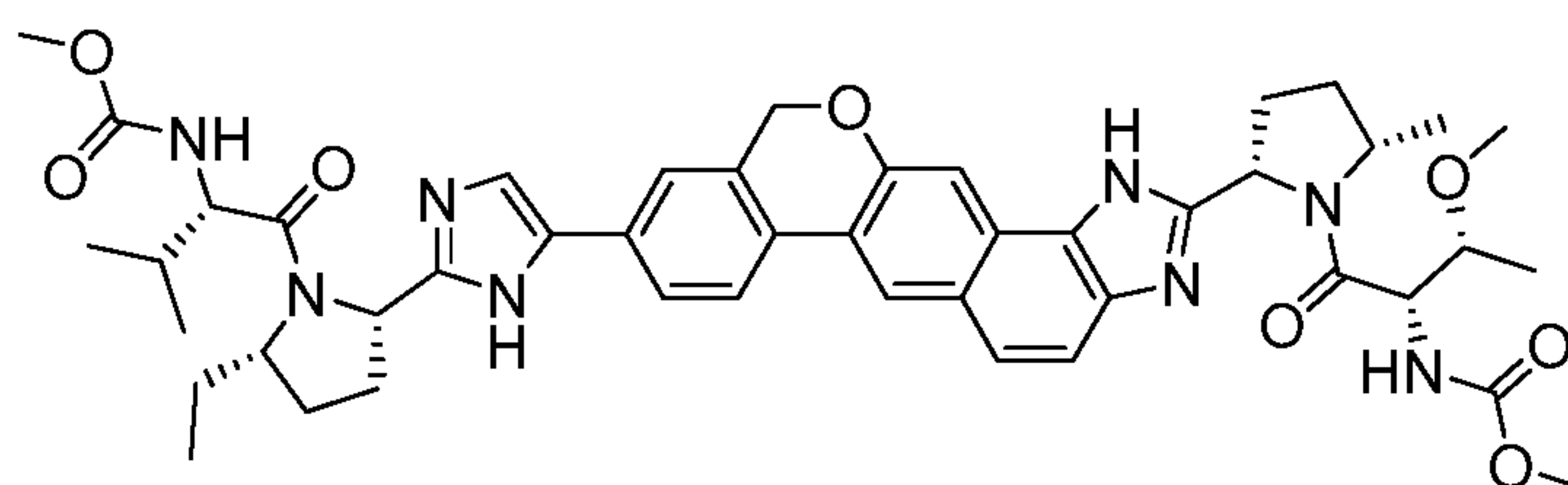
methyl{(2S,3R)-1-[(2S,5S)-2-(9-{2-[(2S,5S)-5-ethyl-1-[(2S)-2-[(methoxycarbonyl) amino]-3-methylbutanoyl]pyrrolidin-2-yl]-1H-imidazol-5-yl}-1,11-dihydroisochromeno[4',3':6,7]naphtho[1,2-d]imidazol-2-yl)-5-methylpyrrolidin-1-yl]-3-methoxy-1-oxobutan-2-yl}carbamate
