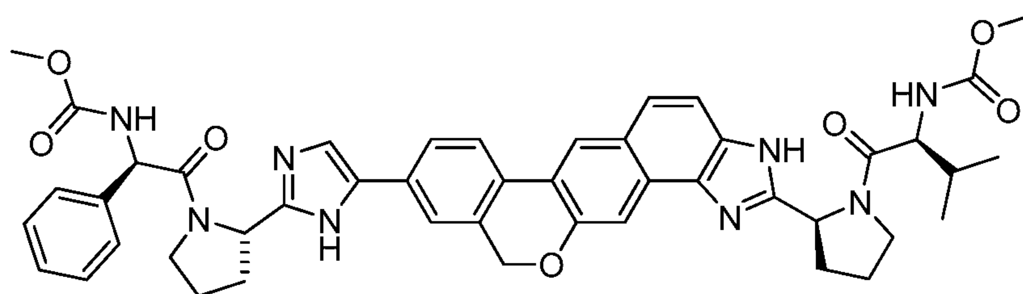
methyl [1-(2-{5-[2-(1-[(methoxycarbonyl)amino]-3-methyl-1-oxobutan-2-yl}pyrrolidin-2-yl)-1,11-dihydroisochromeno[4',3':6,7]naphtho[1,2-d]imidazol-9-yl]-1H-imidazol-2-yl}pyrrolidin-1-yl)-phenyl-1-oxoacet-2-yl]carbamate
