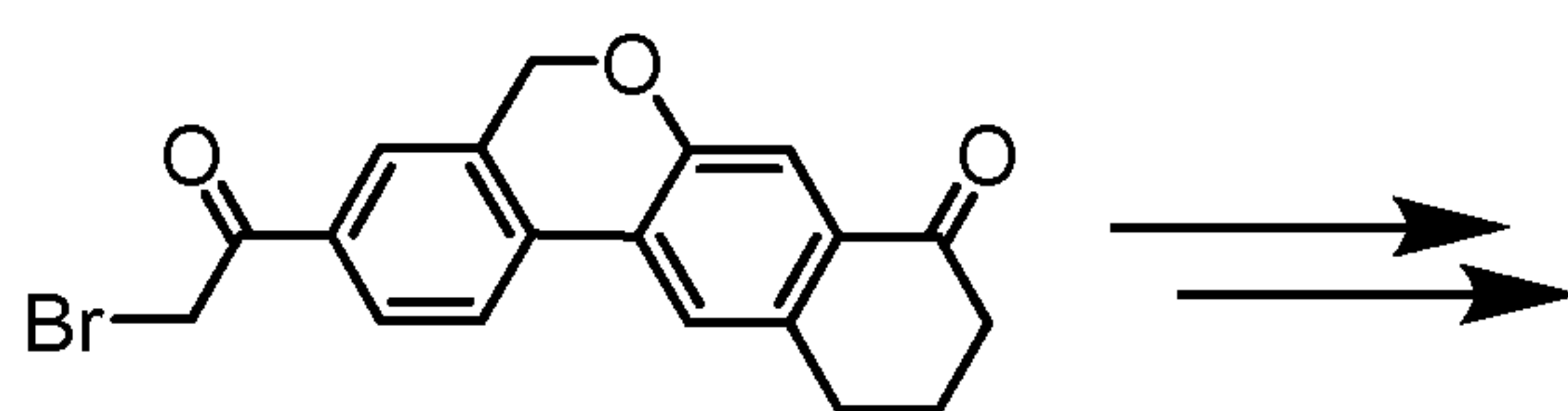
3-(2-bromoacetyl)-10,11-dihydro-5H-dibenzo[c,g]chromen-8(9H)-one
