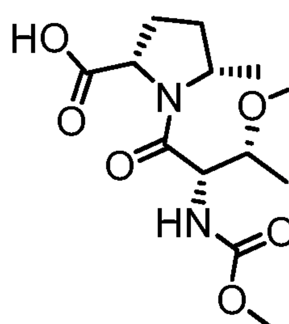
(2S,5S)-1-((2S,3R)-3-methoxy-2-(methoxycarbonylamino)butanoyl)-5-methylpyrrolidine-2-carboxylic acid
