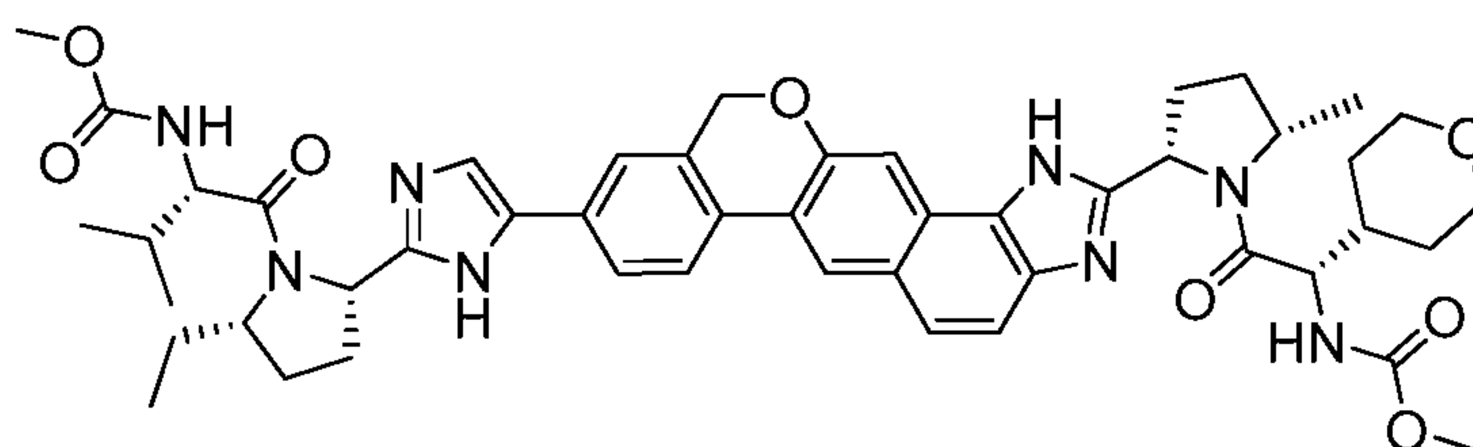
Methyl[(1S)-2-[(2S,5S)-2-(9-{2-[(2S,5S)-5-ethyl-1-{(2S)-2[(methoxycarbonyl)amino]-3-methylbutanoyl}pyrrolidin-2-yl]-1H-imidazol-5-yl}-1,11dihydroisochromeno [4',3':6,7]naphtho[1,2-d]imidazol-2-yl)-5-methylpyrrolidin-1-yl]-2-oxo-1(tetrahydro-2H-pyran-4-yl)ethyl]carbamate
