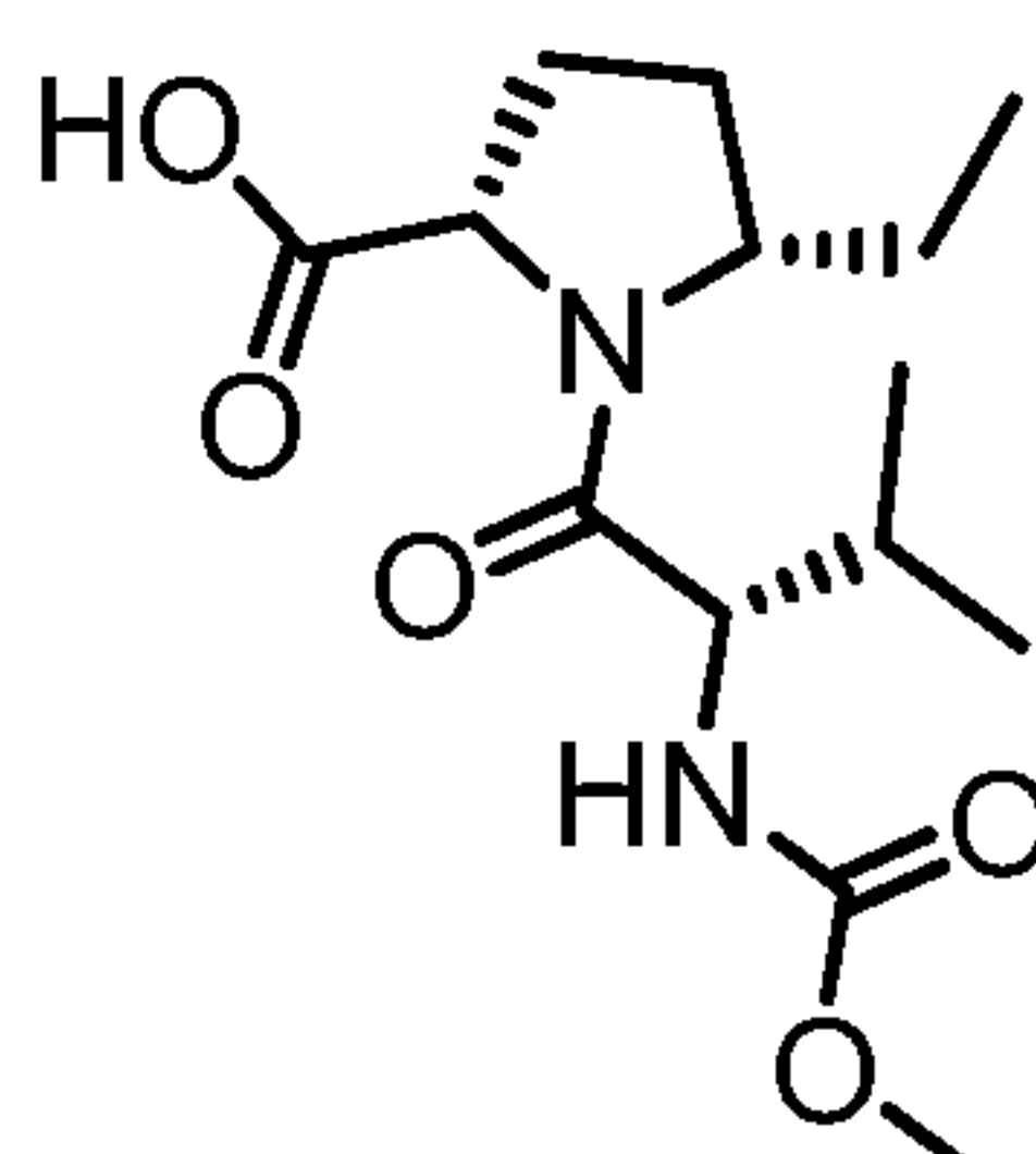
(2S,5S)-5-ethyl-1-((S)-2-(methoxycarbonylamino)-3-methylbutanoyl)pyrrolidine-2-carboxylic acid
