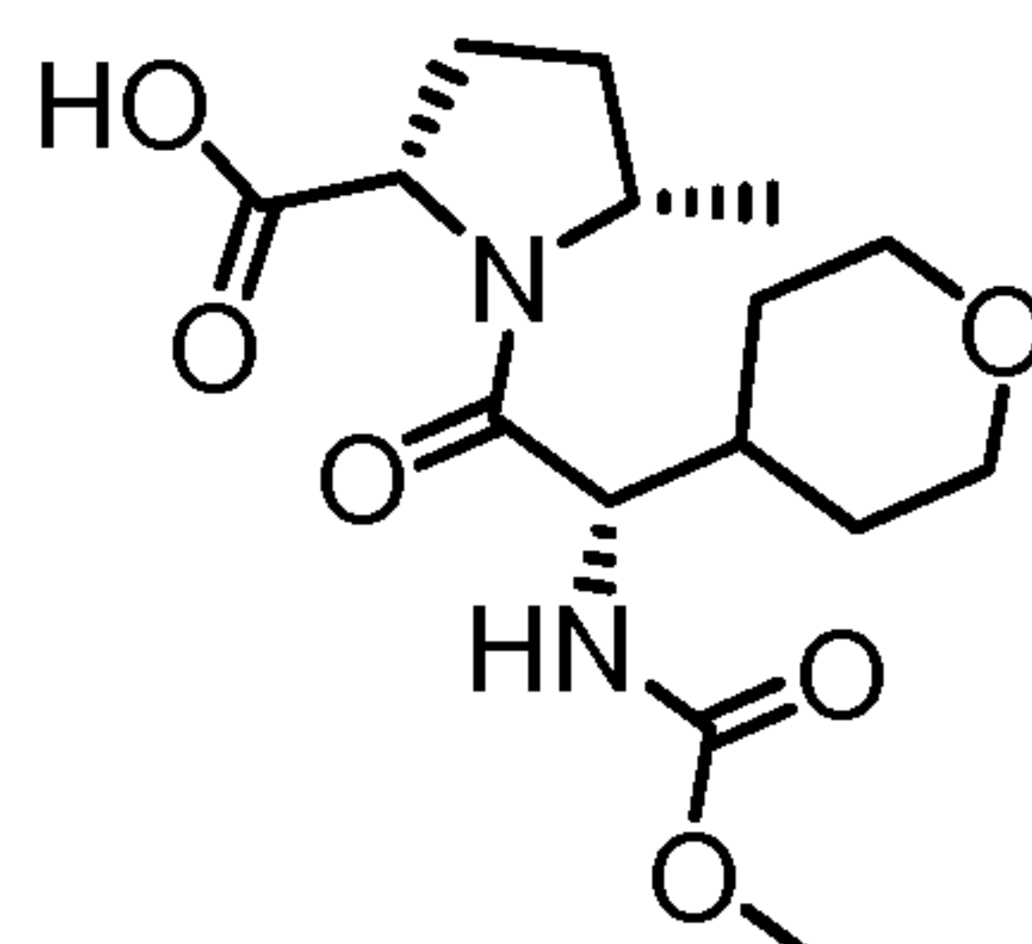
(2S,5S)-1-((S)-2-(methoxycarbonylamino)-2-(tetrahydro-2H-pyran-4-yl)acetyl)-5-methyl pyrrolidine-2-carboxylic acid
