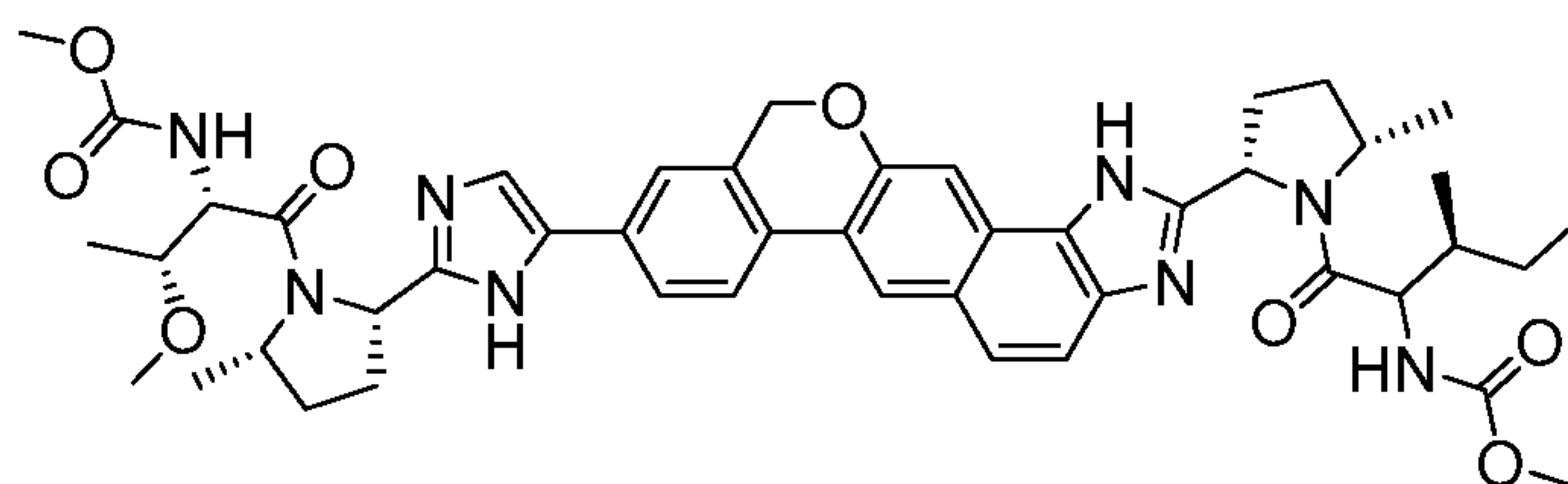
methyl{(3S)-1-[(2S,5S)-2-(9-{2-[(2S,5S)-1-[(2S,3R)-3-methoxy-2-[(methoxycarbonyl) amino]butanoyl]-5-methylpyrrolidin-2-yl]-1H-imidazol-5-yl}-1,11-dihydroisochromeno[4',3':6,7]naphtho[1,2-d]imidazol-2-yl)-5-methylpyrrolidin-1-yl]-3-methyl-1-oxopentan-2-yl}carbamate
