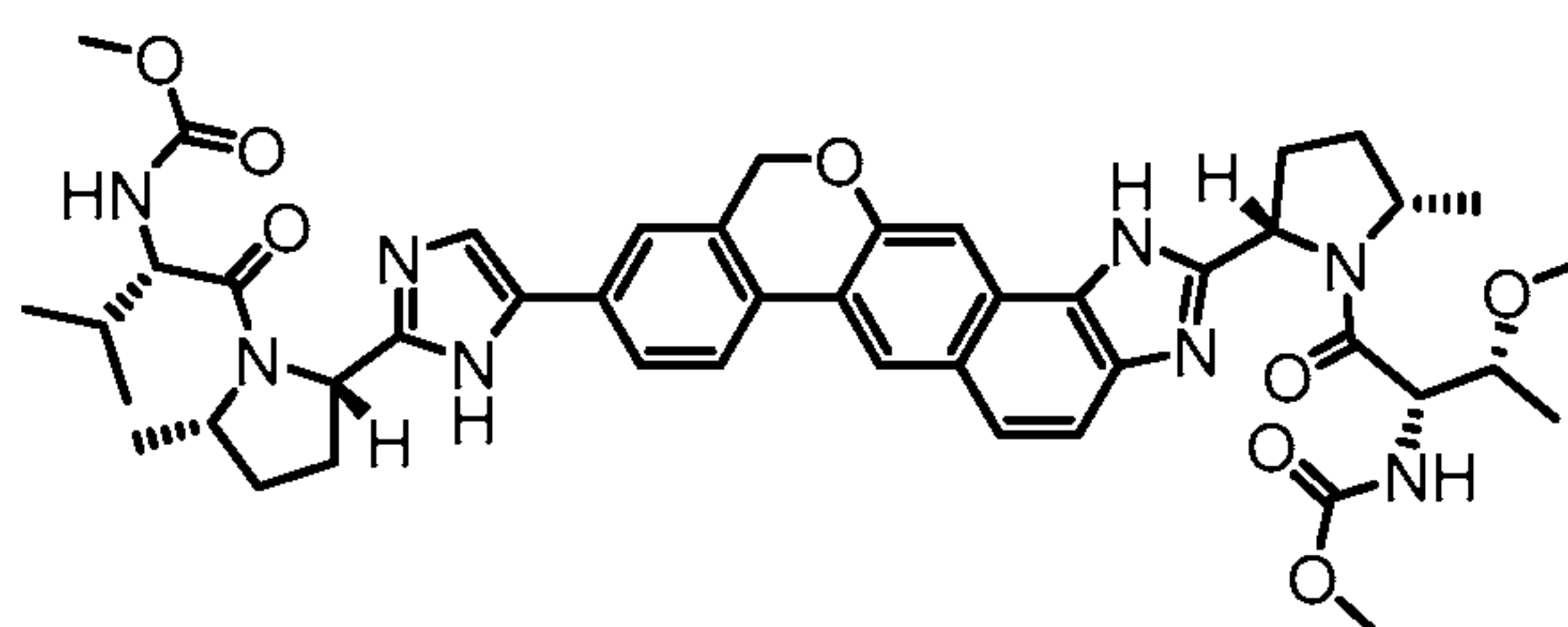
methyl [(2S)-1-[(2S,5S)-2-[5-(2-[(2S,5S)-1-[N-(methoxycarbonyl)-O-methyl-L-threonyl]-5-methylpyrrolidin-2-yl]-1,11-dihydroisochromeno[4',3':6,7]naphtho[1,2-d]imidazol-9-yl)-1H-imidazol-2-yl]-5-methylpyrrolidin-1-yl]-3-methyl-1-oxobutan-2-yl]carbamate 15
