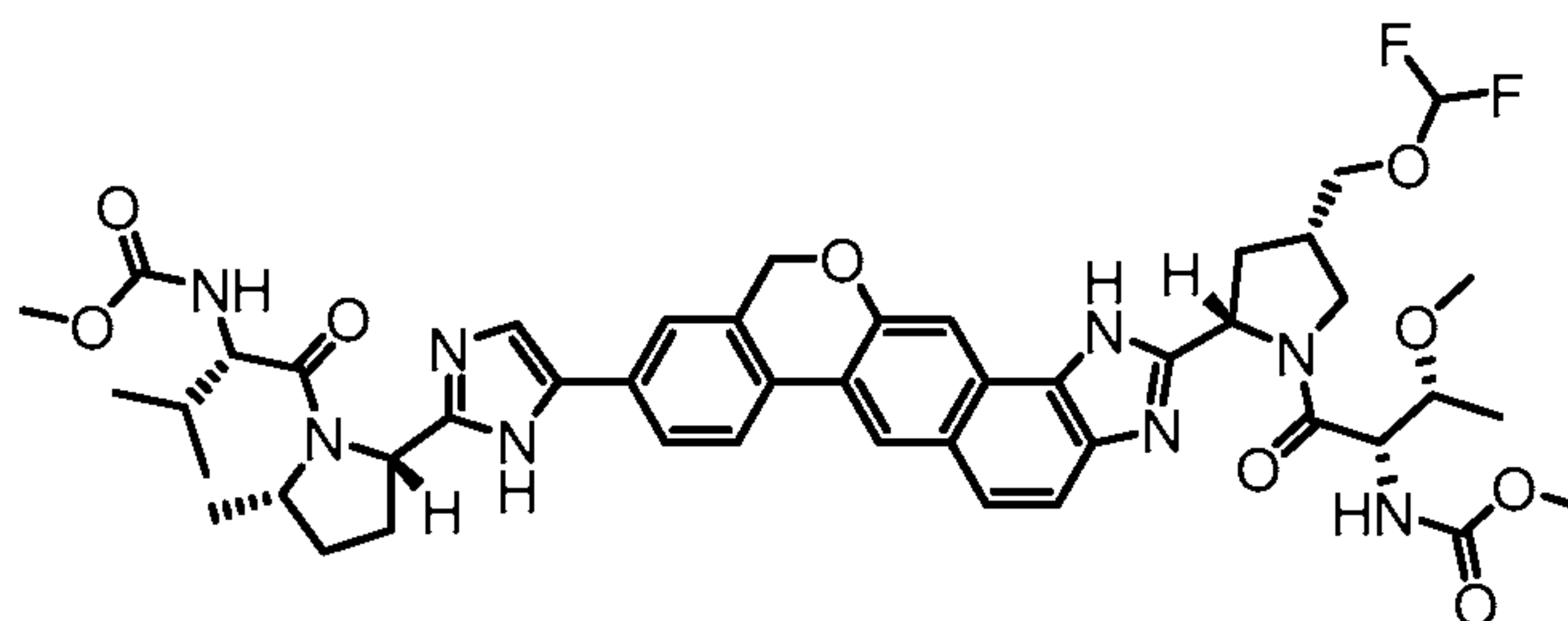
methyl [(2S,3R)-1-[(2S,4S)-4-[(difluoromethoxy)methyl]-2-[9-(2-[(2S,5S)-1-[N-(methoxycarbonyl)-L-valyl]-5-methylpyrrolidin-2-yl]-1H-imidazol-5-yl)-1,11-dihydroisochromeno[4',3':6,7]naphtho[1,2-d]imidazol-2-yl]pyrrolidin-1-yl]-3-methoxy-1-oxobutan-2-yl]carbamate
