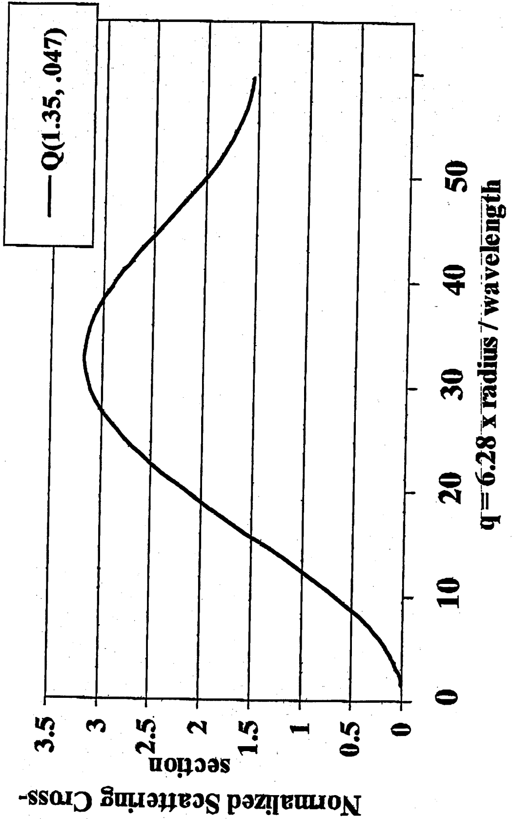
Figure 6 Normalized Scattering Cross-section for Blood
