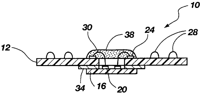
Fig. 3 (PRIOR ART)
