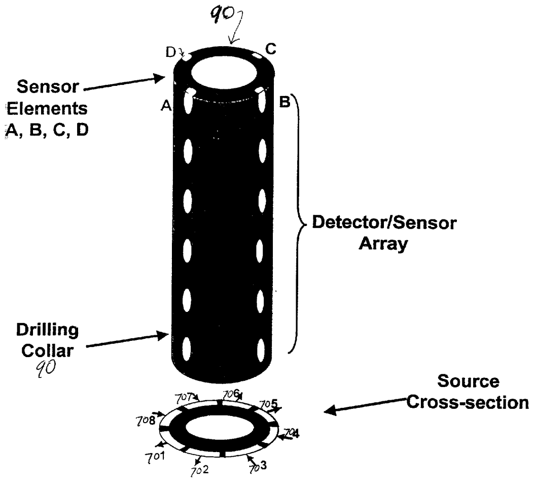
Figure 10 Sensor Array Layout
