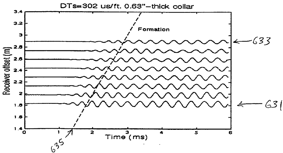
Figure 6B Quadrupole waveforms, thin collar pipe
