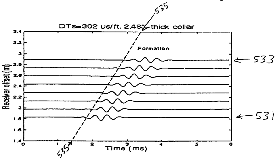
Figure 5B Quadrupole waveforms at various offsets
