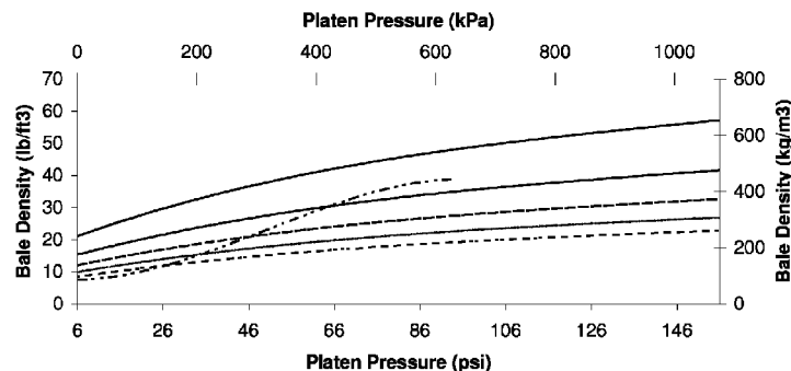
Platen Pressure vs Bale Density
