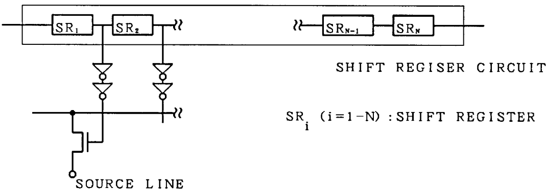
Fig 5 (prior art)
