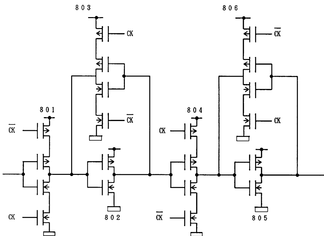
Fig. 8 (Prior Art)
