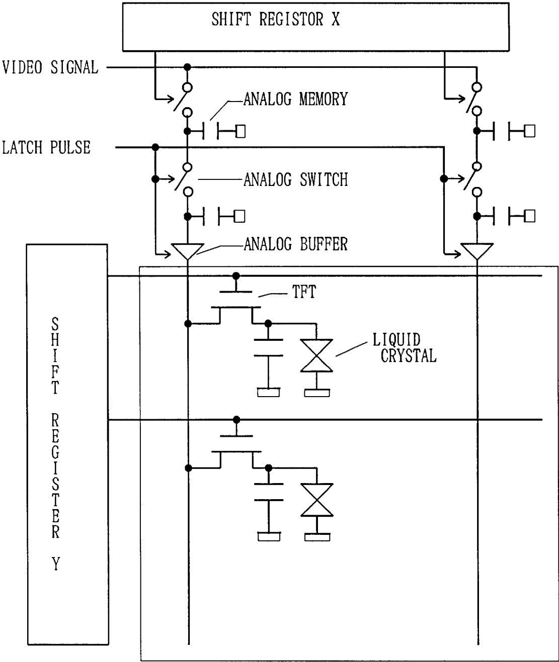
Fig. 6 (prior art)
