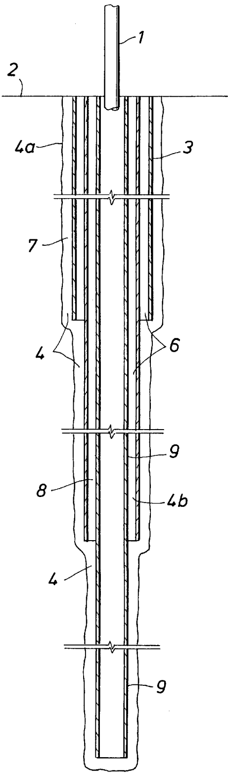
FIG. 1 (PRIOR ART)
