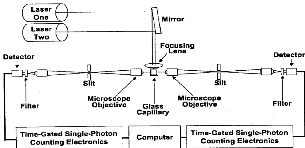
Schematic diagram of the basic apparatus for single molecule detection using laser induced fluorescence.
