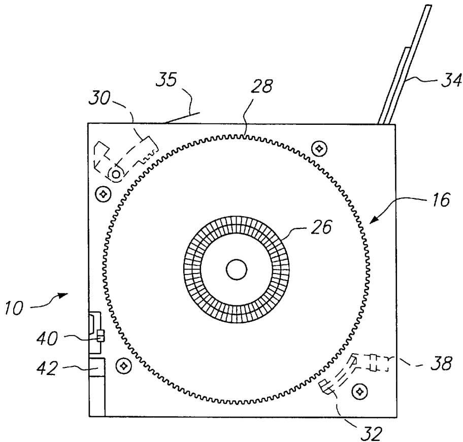
FIG. 2 (PRIOR ART)
