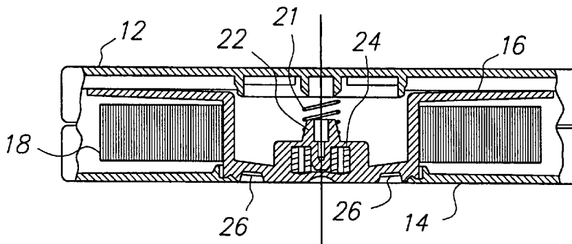
FIG. 3 (PRIOR ART)
