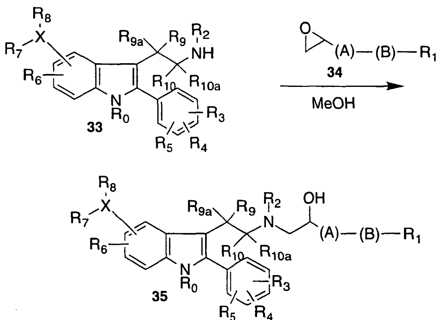
Reaction Scheme M
