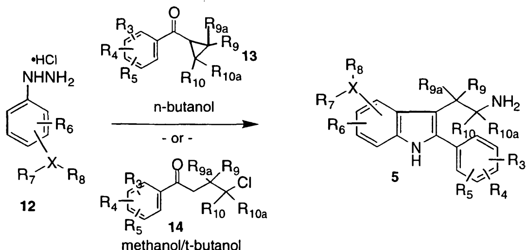
Reaction Scheme E
