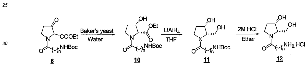
Scheme 2. Synthesis of cis-(2R,3S)-pyrrolidine diol
