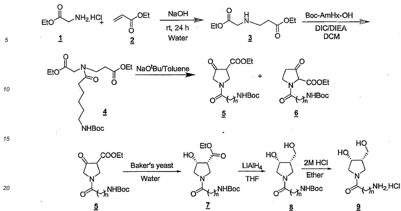
Scheme 1. Synthesis of cis-(2S,4R)-pyrrolidine diol
