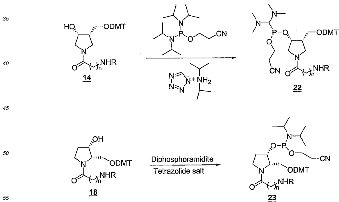
Scheme 4 Cholesterol conjugation at 3'-end with 2R,3S pyrrolidiny derivative
