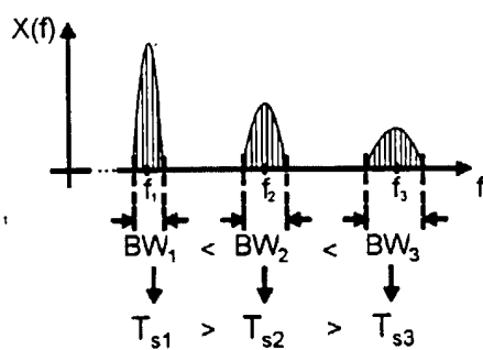
Figure 24: Spectral representation of an MRMC signal.
