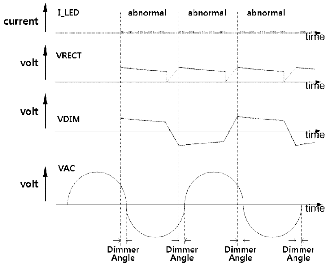
FIG.4 Prior Art
