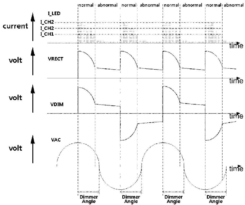
FIG.3 Prior Art
