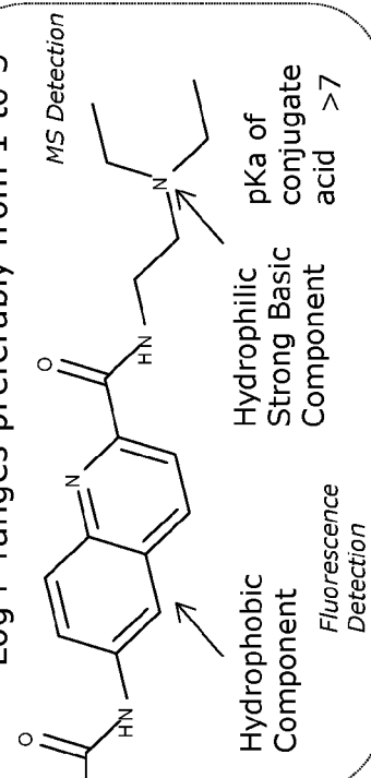
FIG. 1. Example chemical structure of a glycan modified with an amphipathic, strongly basic moiety. A heptasaccharide glycan labeled with RFMS.
