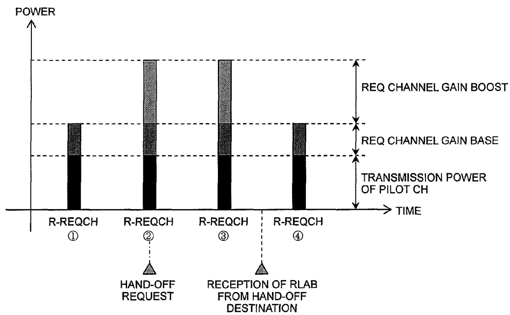
POWER FLUCTUATION OF R-REQCH (REVERSE LINK)
