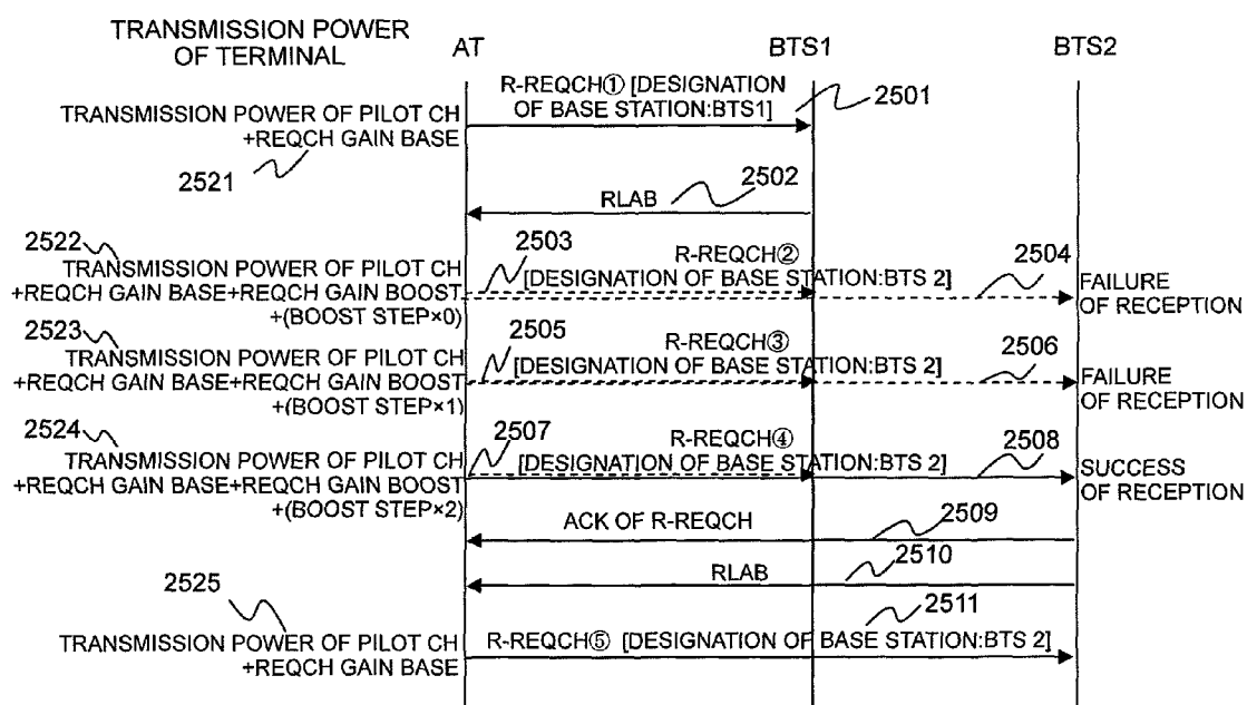
POWER CONTROL ALGORITHM OF R-REQCH (REVERSE LINK)
