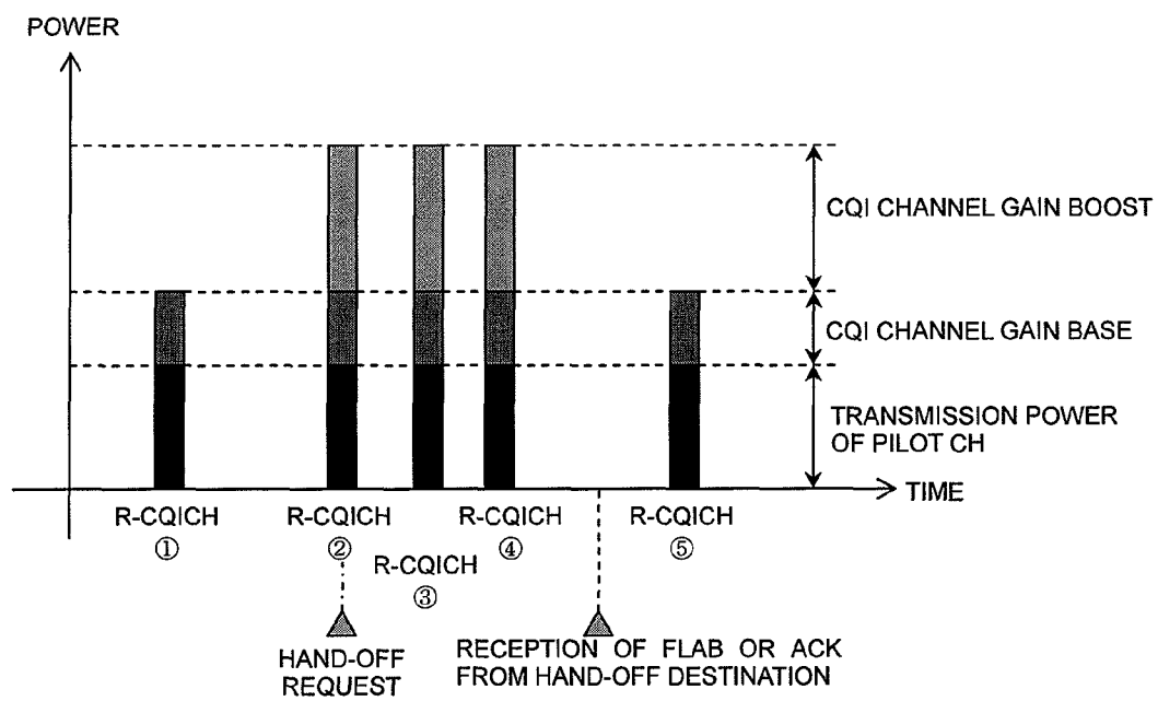
POWER FLUCTUATION OF R-CQICH (FORWARD LINK)
