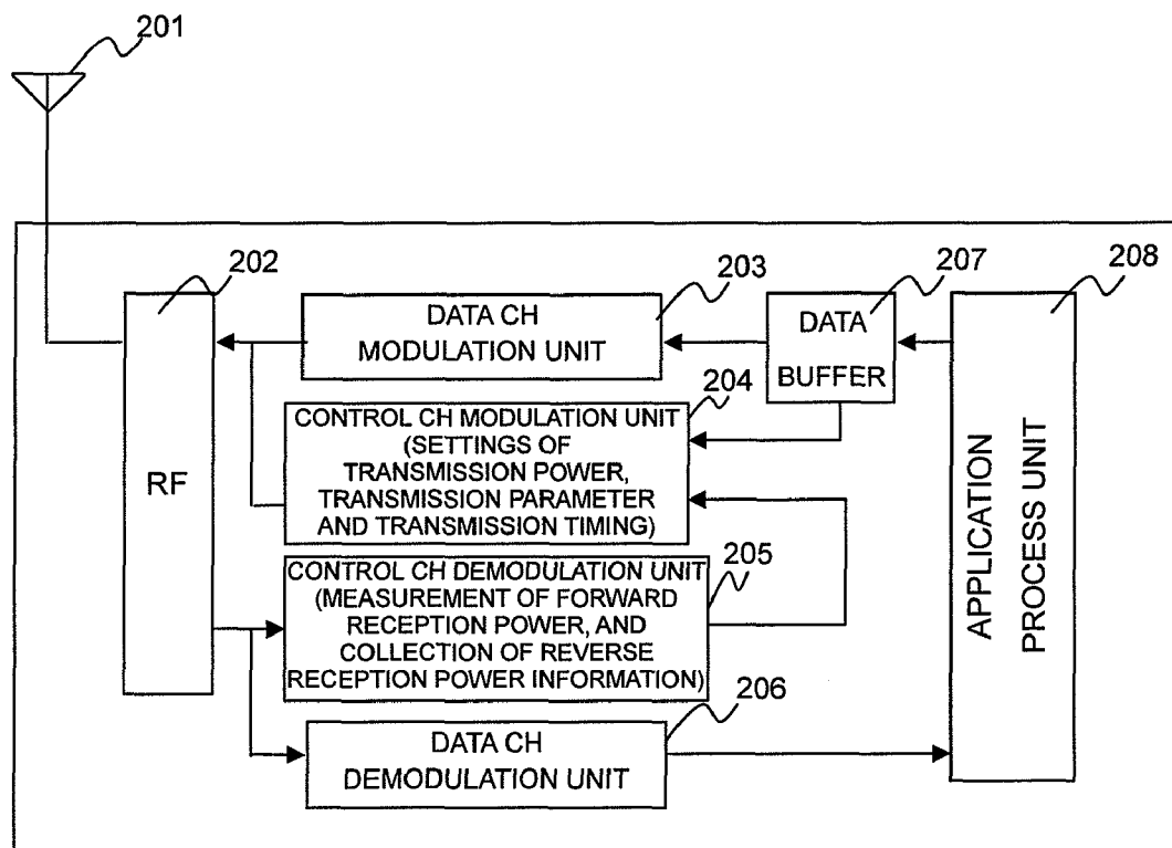
CONFIGURATION OF RADIO ACCESS TERMINAL
