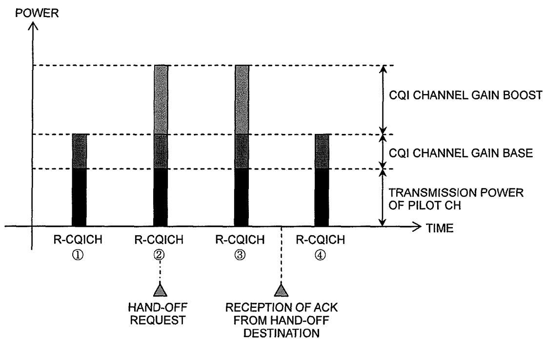
POWER FLUCTUATION OF R-CQICH (FORWARD LINK)
