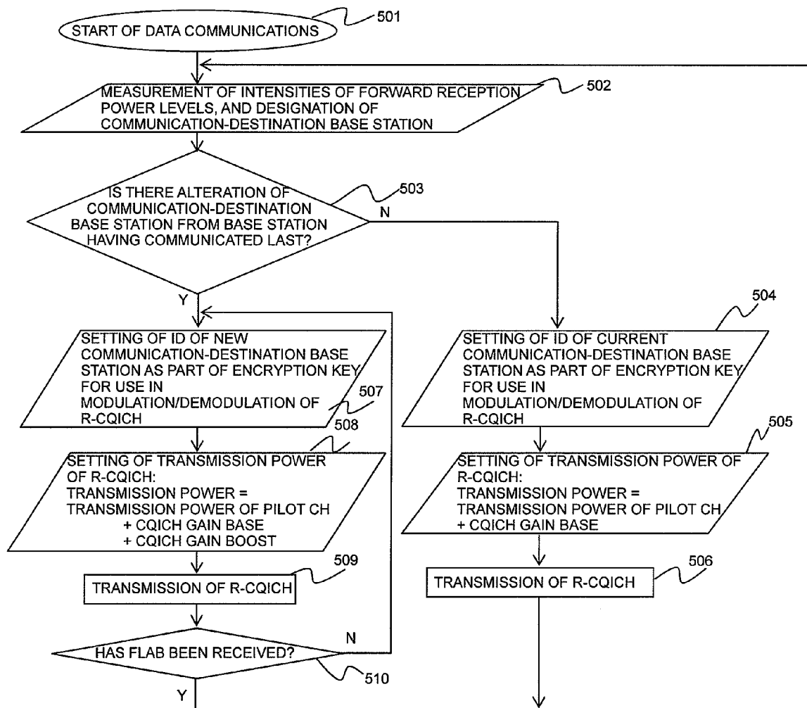
FLOW CHART OF "AT" IN FIRST EMBODIMENT (FORWARD LINK)
