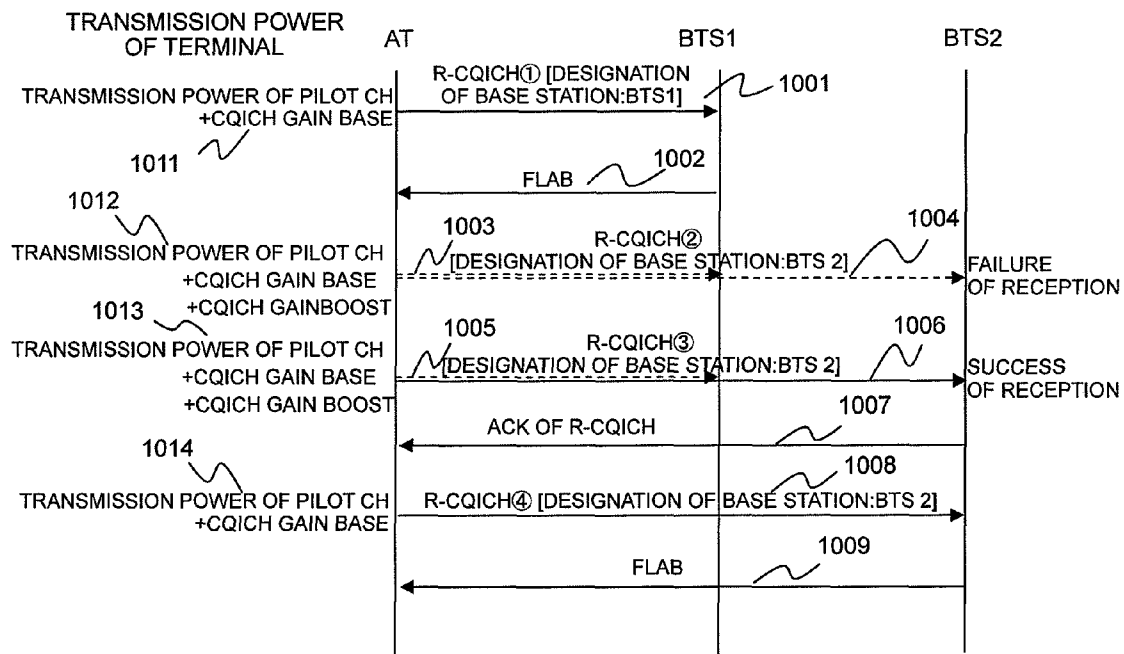
POWER CONTROL ALGORITHM OF R-CQICH (FORWARD LINK)
