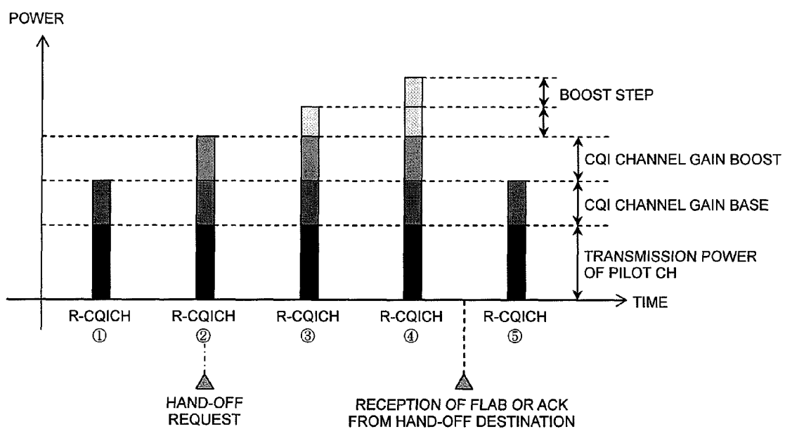
POWER FLUCTUATION OF R-CQICH (FORWARD LINK)
