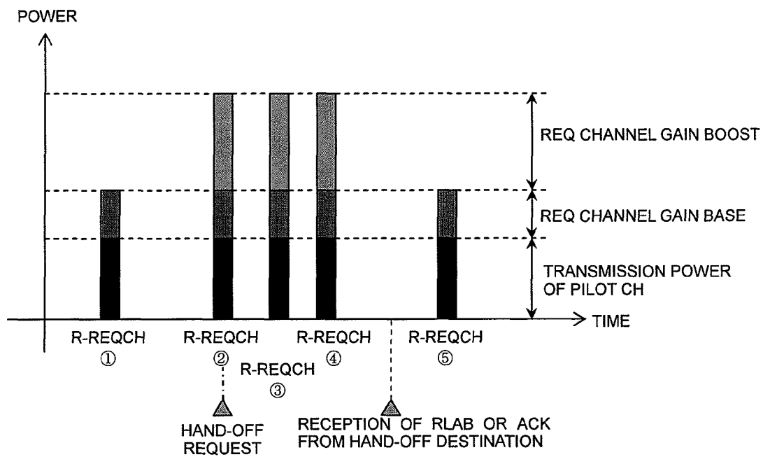
POWER FLUCTUATION OF R-REQCH (REVERSE LINK)
