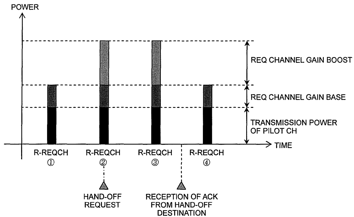
POWER FLUCTUATION OF R-REQCH (REVERSE LINK)
