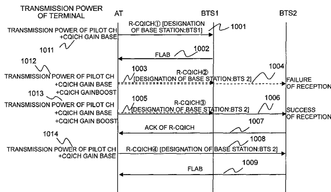
POWER CONTROL ALGORITHM OF R-CQICH (FORWARD LINK)
