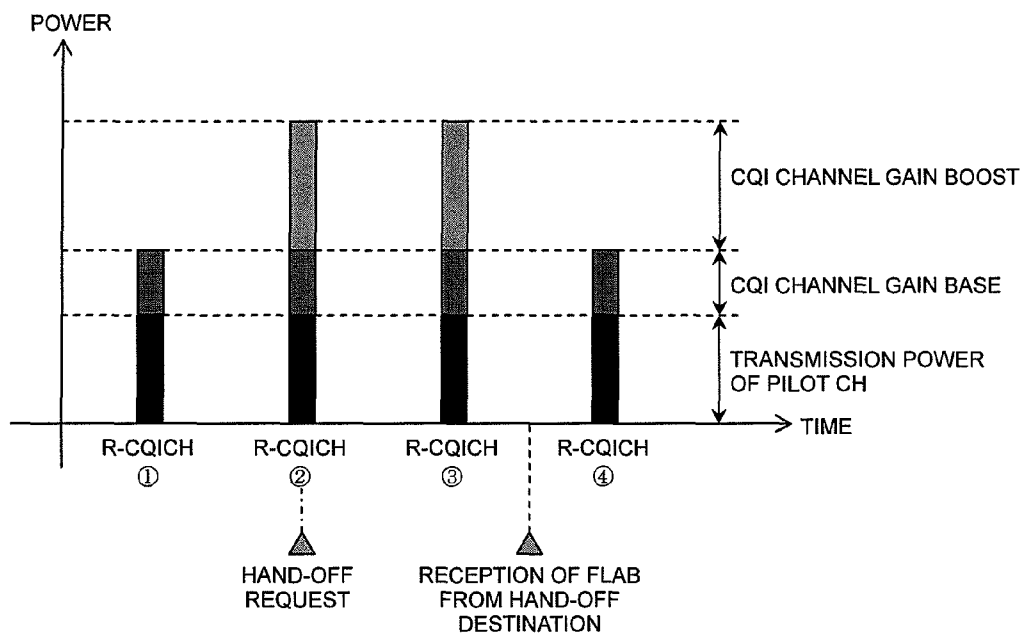
POWER FLUCTUATION OF R-CQICH (FORWARD LINK)
