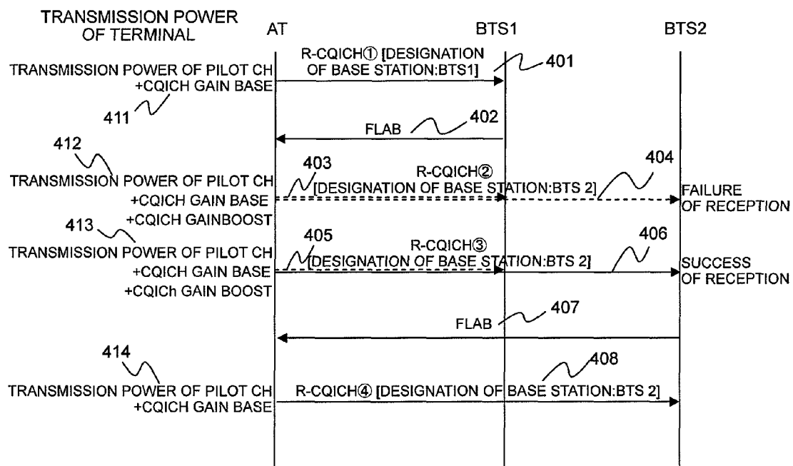
POWER CONTROL ALGORITHM OF R-CQICH (FORWARD LINK)
