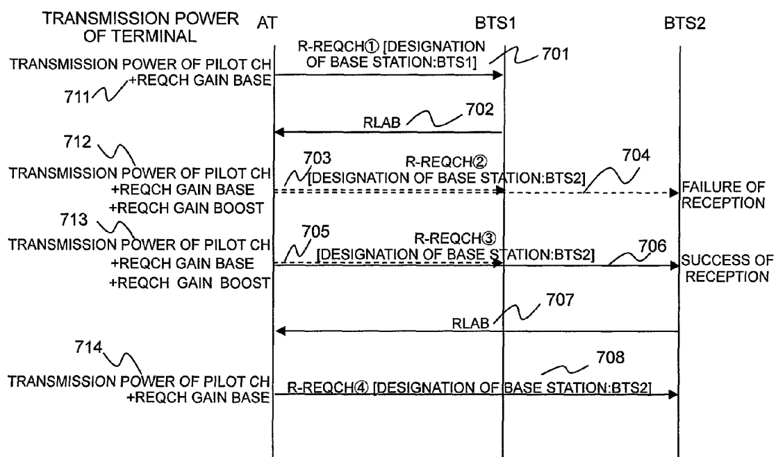
POWER CONTROL ALGORITHM OF R-REQCH (REVERSE LINK)
