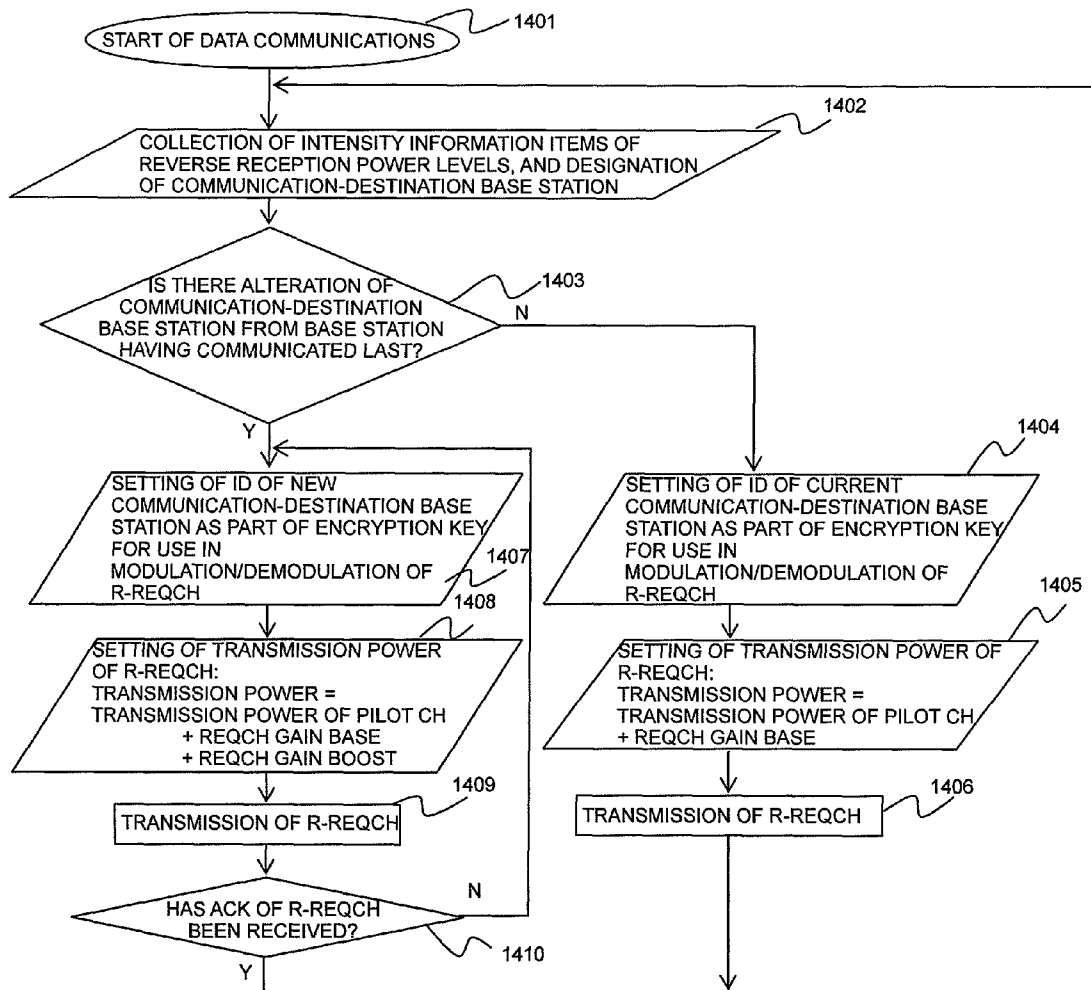
FLOW CHART OF "AT" IN SECOND EMBODIMENT (REVERSE LINK)
