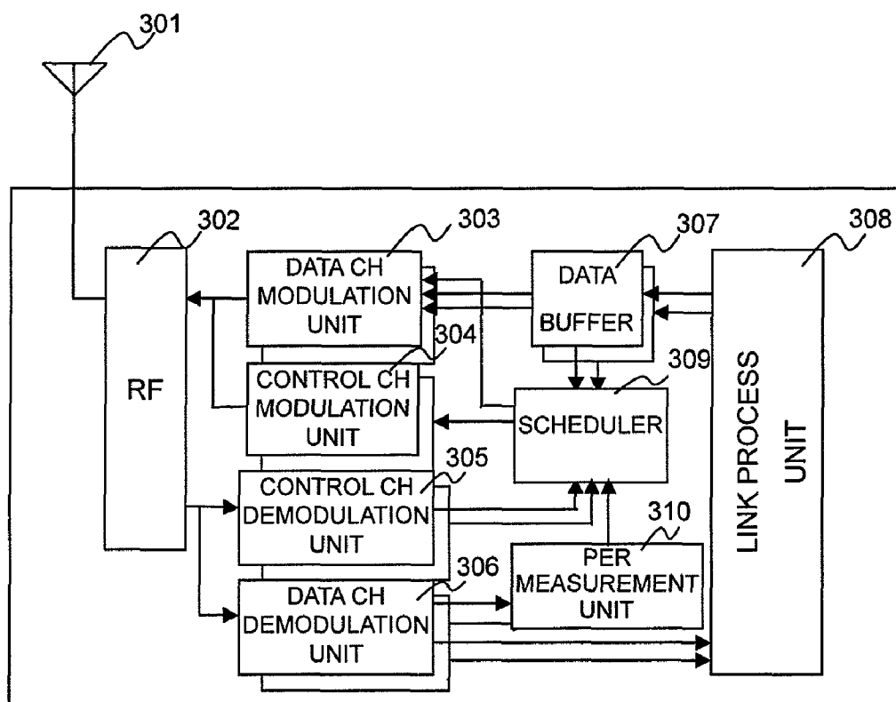
CONFIGURATION OF RADIO BASE STATION
