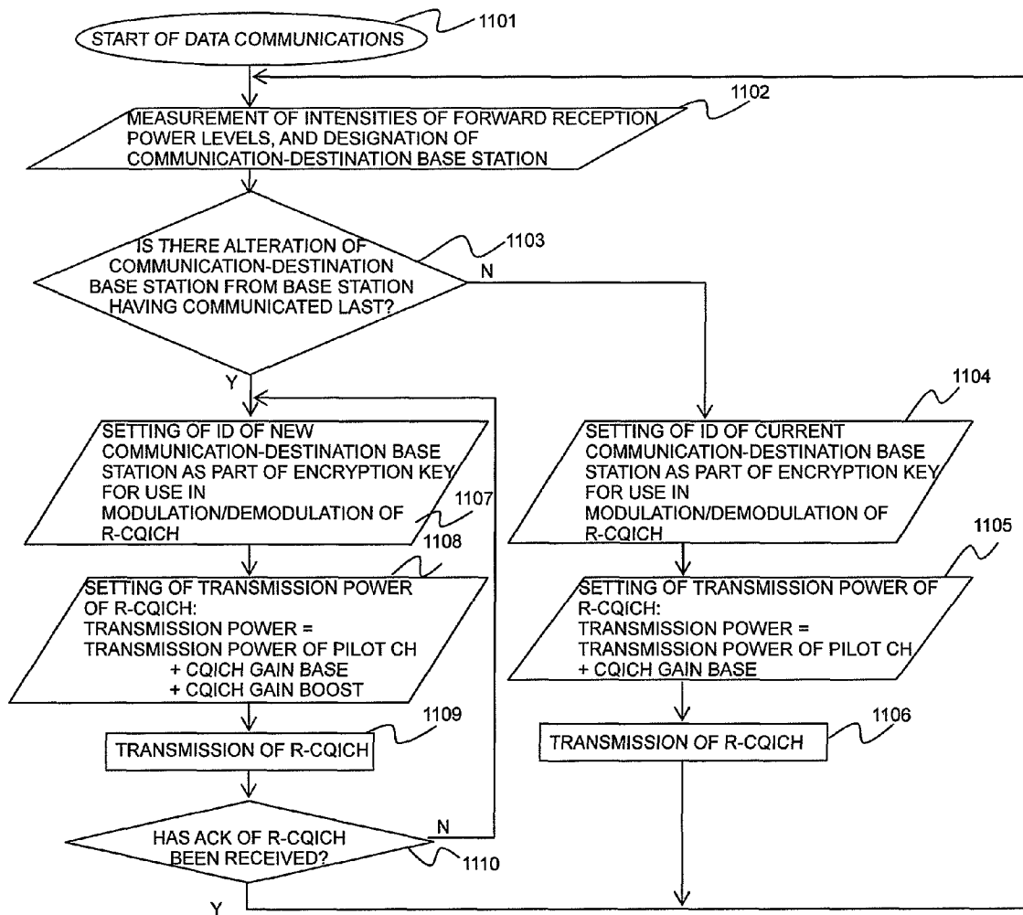
FLOW CHART OF "AT" IN SECOND EMBODIMENT (FORWARD LINK)
