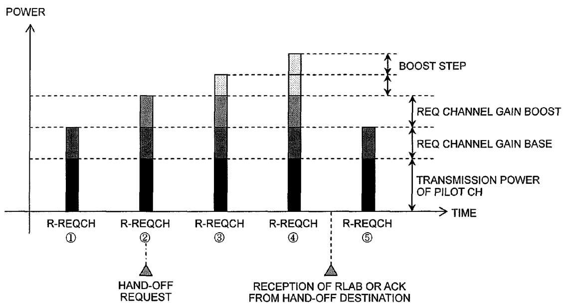
POWER FLUCTUATION OF R-REQCH (REVERSE LINK)
