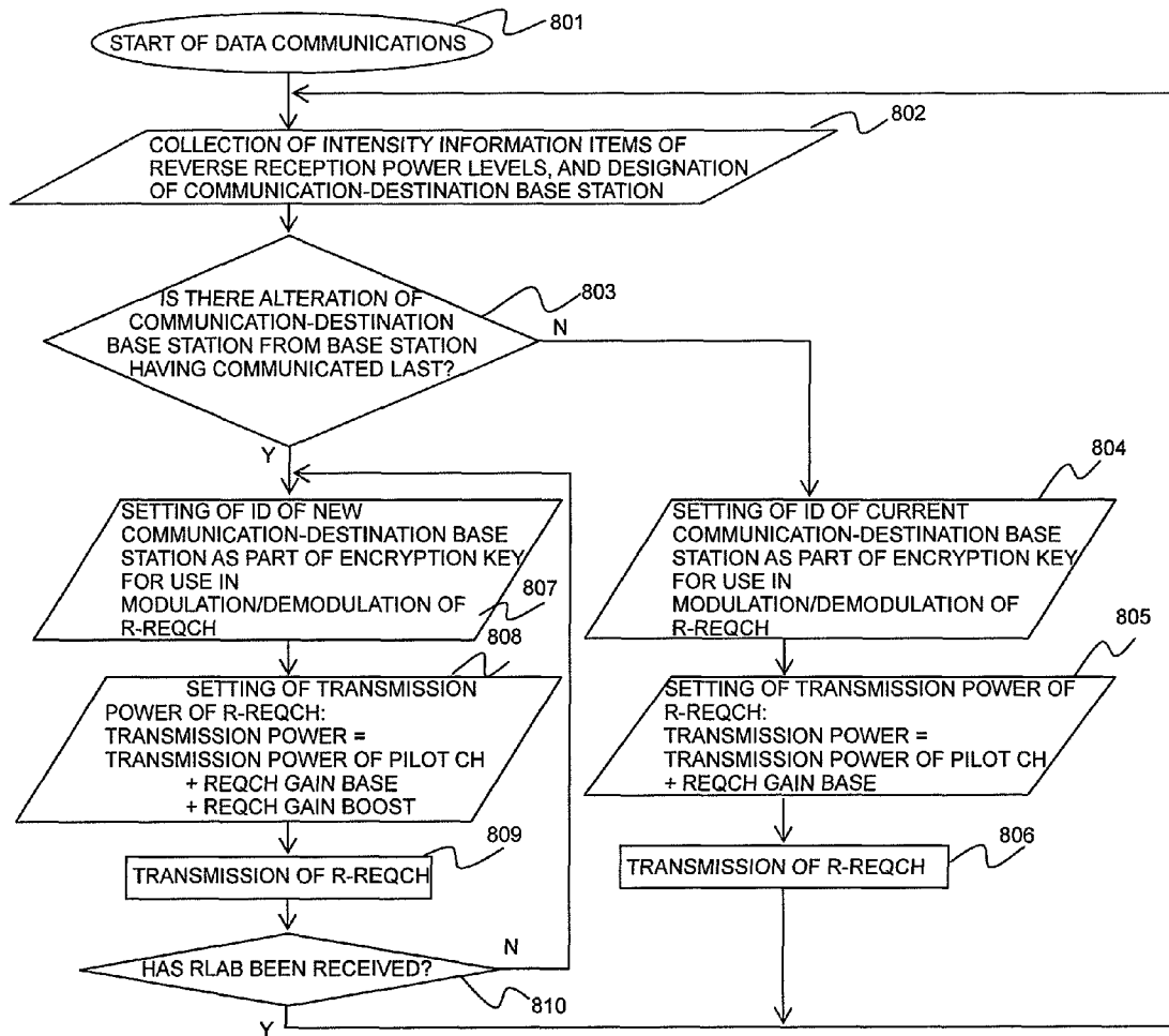
FLOW CHART OF "AT" IN FIRST EMBODIMENT (REVERSE LINK)
