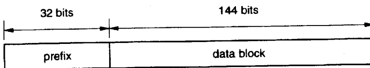
FIG. 5 (PRIOR ART)
