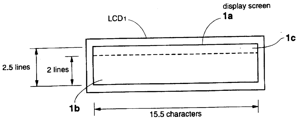
FIG. 7 (PRIOR ART)
