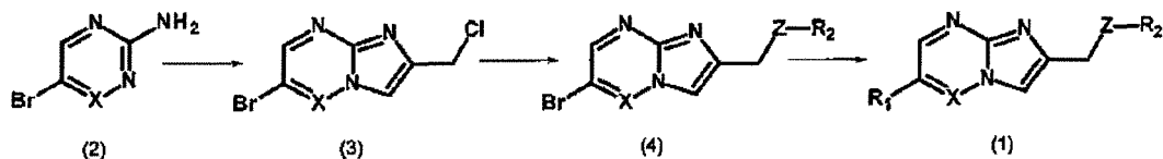
[Reaction Scheme 1]
