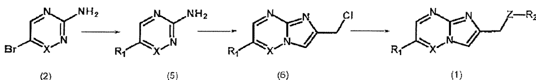
[Reaction Scheme 2]
