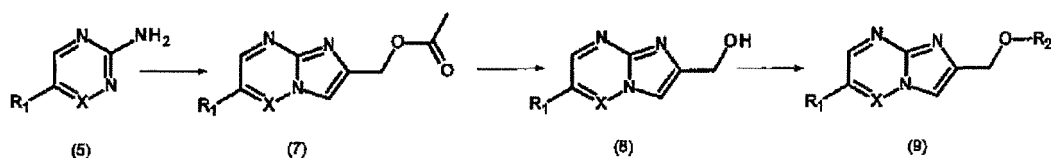
[Reaction Scheme 3]
