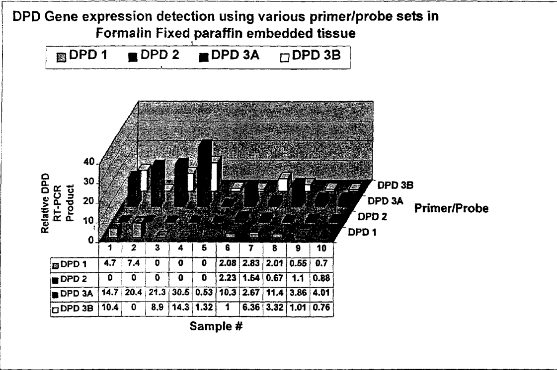
Fig. 1. Comparison of 4 DPD primer/probe sets for their ability to amplify DPD mRNA.
