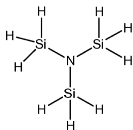
Trisilylamine (TSA)
