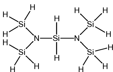
Bis(disilylamino)silane
