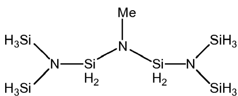
Bis[bis(silyl)amino)silyl]methanamine
