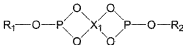
[Chemical Formula 1]
