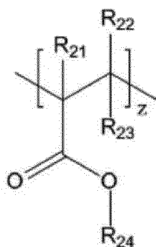
[Chemical Formula 5]
