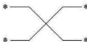
[Chemical Formula 1-1]
