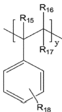
[Chemical Formula 4]
