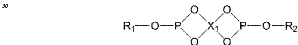
[Chemical Formula 1]
