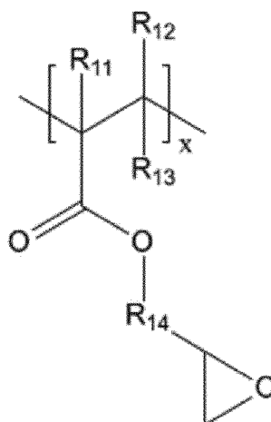
[Chemical Formula 3]
