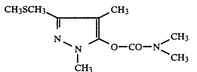
1,4-Dimethyl-5-[N,N-(dimethyl)-carbamoyloxy]-3-methylthio-methyl-pyrazole
