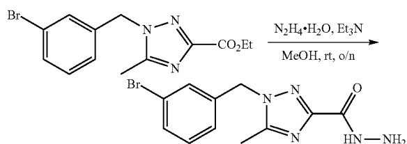
1-(3-Bromobenzyl)-5-methyl-1H-1,2,4-triazole-3-carbohydrazide
