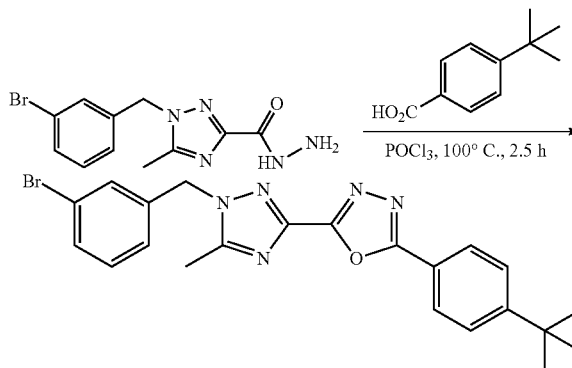
2-(1-(3-Bromobenzyl)-5-methyl-1H-1,2,4-triazol-3-yl)-5-(4-(tert-butyl)phenyl)-1,3,4-oxadiazole
