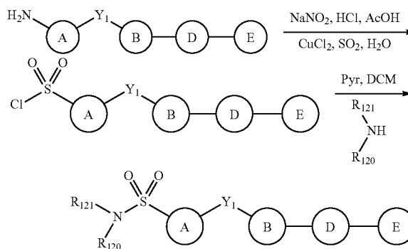
Scheme 11:
