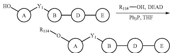
Scheme 9b
