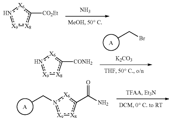
SCHEME 13:
