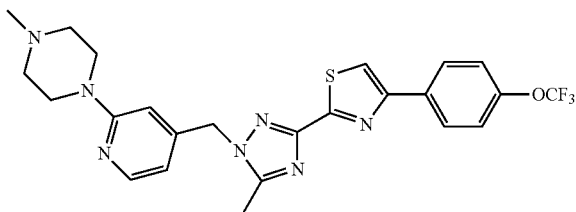
2-(5-methyl-1-((2-(4-methylpiperazin-1-yl)pyridin-4-yl)methyl)-1H-1,2,4-triazol-3-yl)-4-(4-(trifluoromethoxy)phenyl)thiazole
