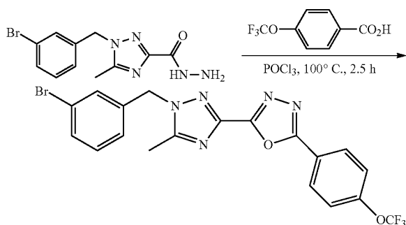
2-(1-(3-Bromobenzyl)-5-methyl-1H-1,2,4-triazol-3-yl)-5-(4-(trifluoromethoxy)phenyl)-1,3,4-oxadiazole
