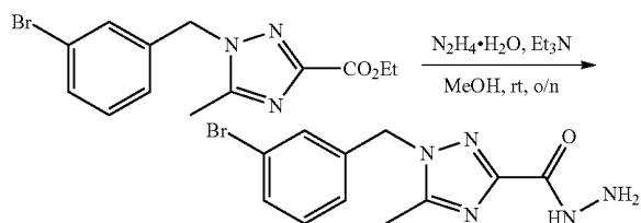
1-(3-Bromobenzyl)-5-methyl-1H-1,2,4-triazole-3-carbohydrazide
