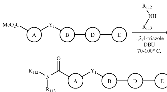
SCHEME 8:
