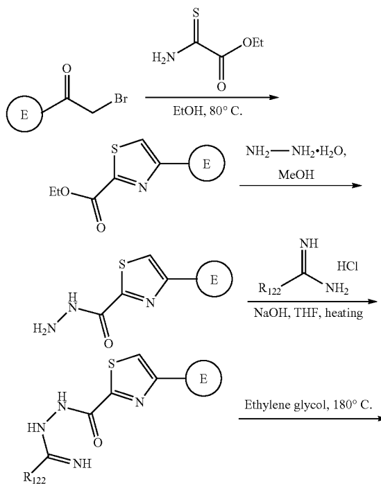
SCHEME 14:
