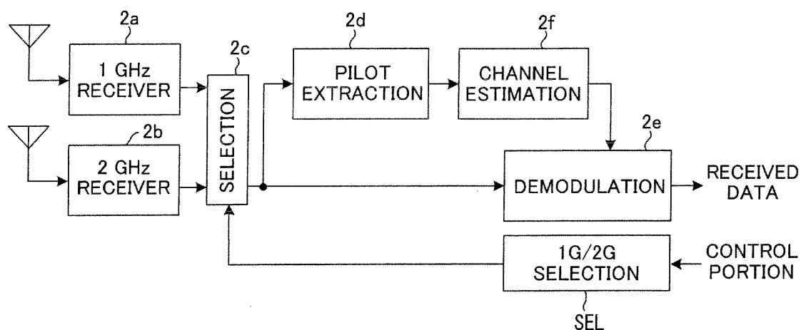
FIG. 18 PRIOR ART
