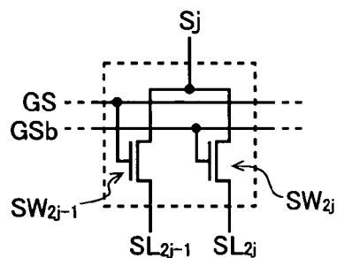
Fig. 2C PRIOR ART
