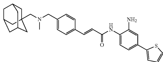
(E)-3-(4-(((3r,5r,7r)-adamantan-1-ylmethyl)(methyl)amino)methyl)phenyl)-N-(2-amino-4-(thiophen-2-yl)phenyl)acrylamide Exact Mass: 511.266 Molecular Weight: 511.721
