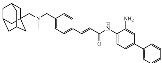
(E)-3-(4-(((3r,5r,7r)-adamantan-1-ylmethyl)(methyl)amino)methyl)phenyl)-N-(3-amino-[1,1-biphenyl]-4-yl)acrylamide Exact Mass: 505.309 Molecular Weight: 505.693
