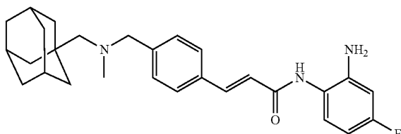
(E)-3-(4-(((3r,5r,7r)-adamantan-1-ylmethyl)(methyl)amino)methyl)phenyl)-N-(2-amino-4-fluorophenyl)acrylamide Exact Mass: 447.269 Molecular Weight: 447.587
