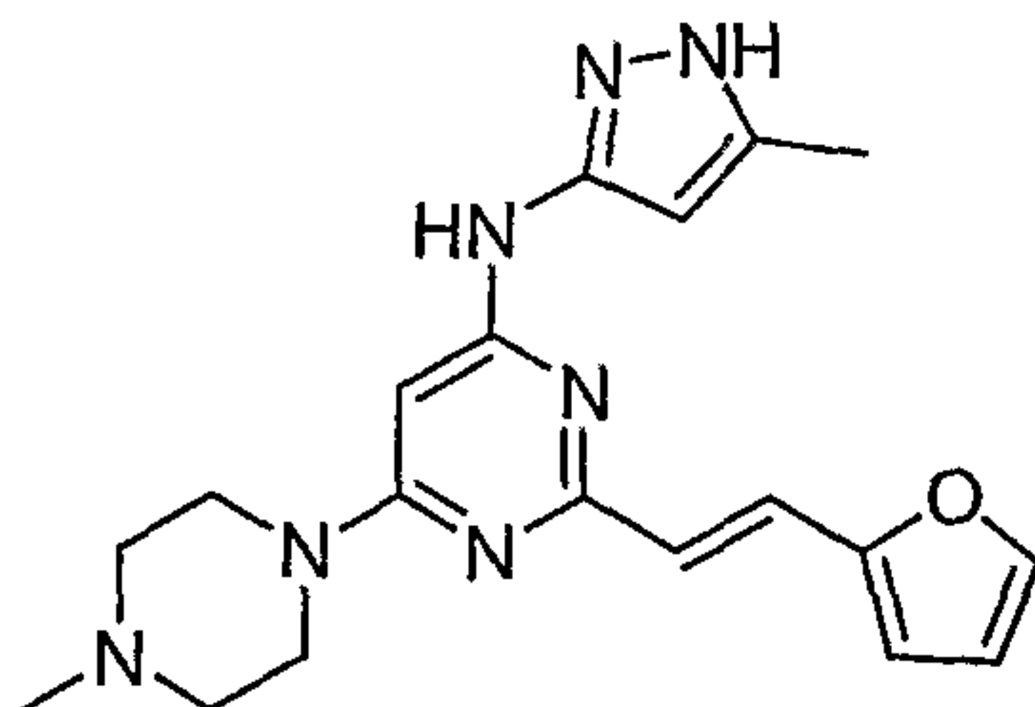
2-((E)-2-(furan-2-yl)vinyl)-N-(5-methyl-1H-pyrazol-3-yl)- 6-(4-methylpiperazin-1-yl)pyrimidin-4-amine
