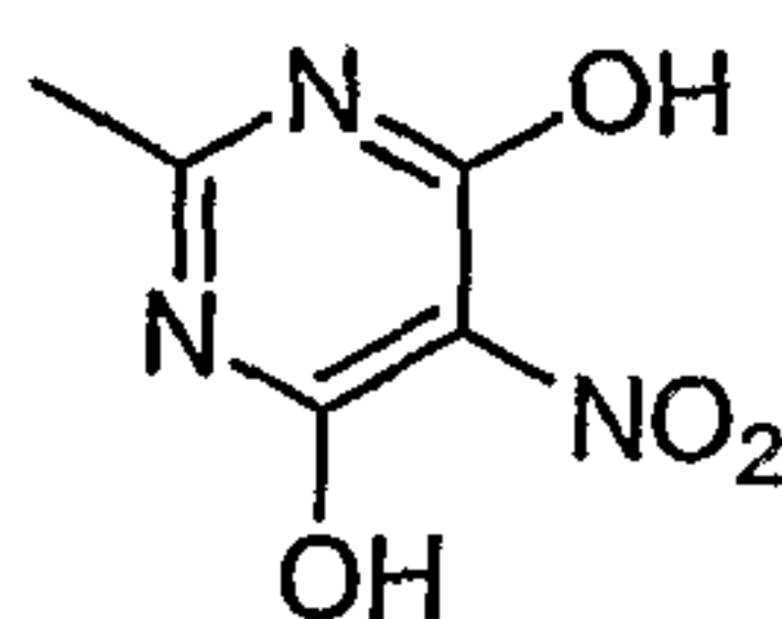
2-methyl-5-nitropyrimidine-4,6-diol
