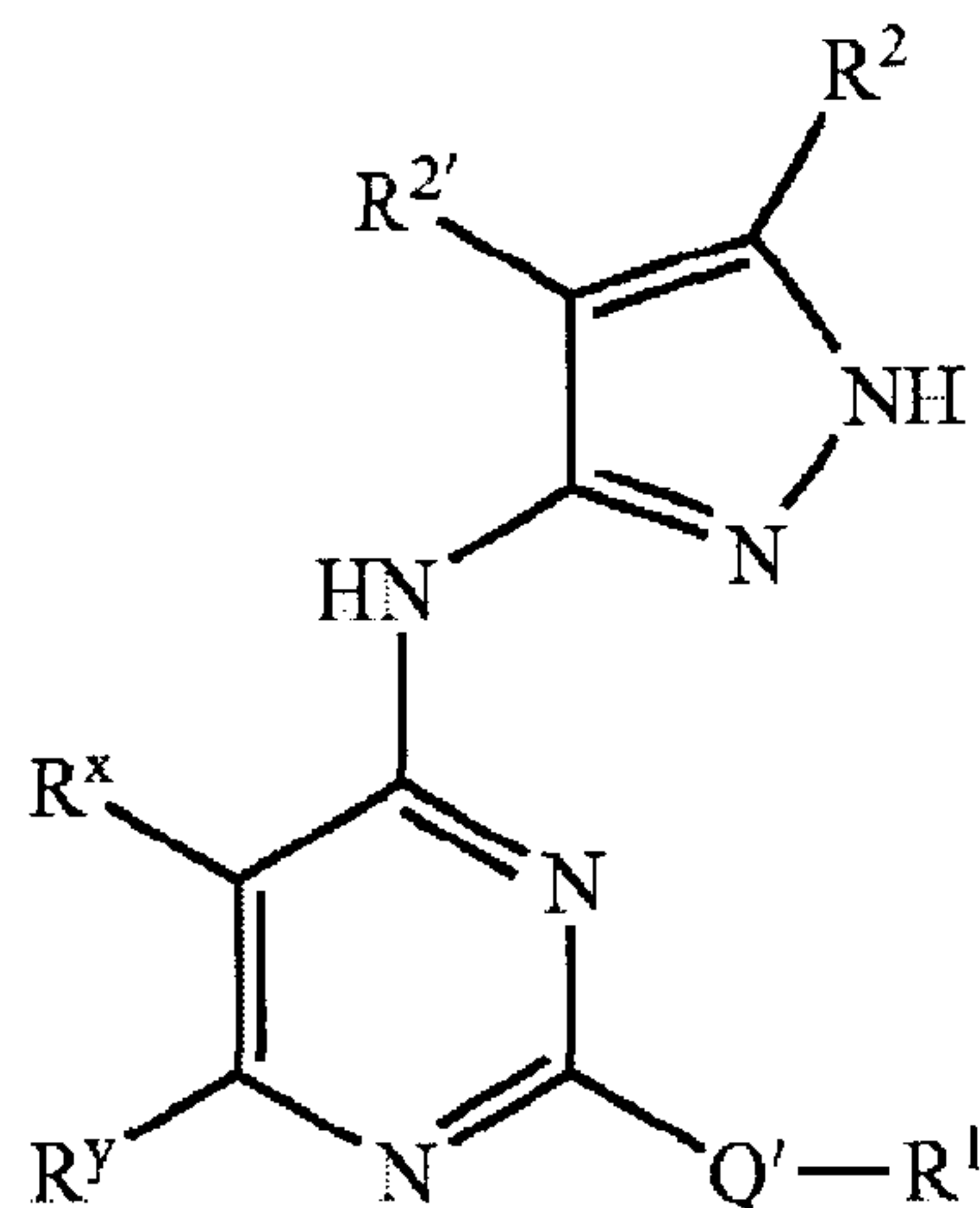
Formula I
