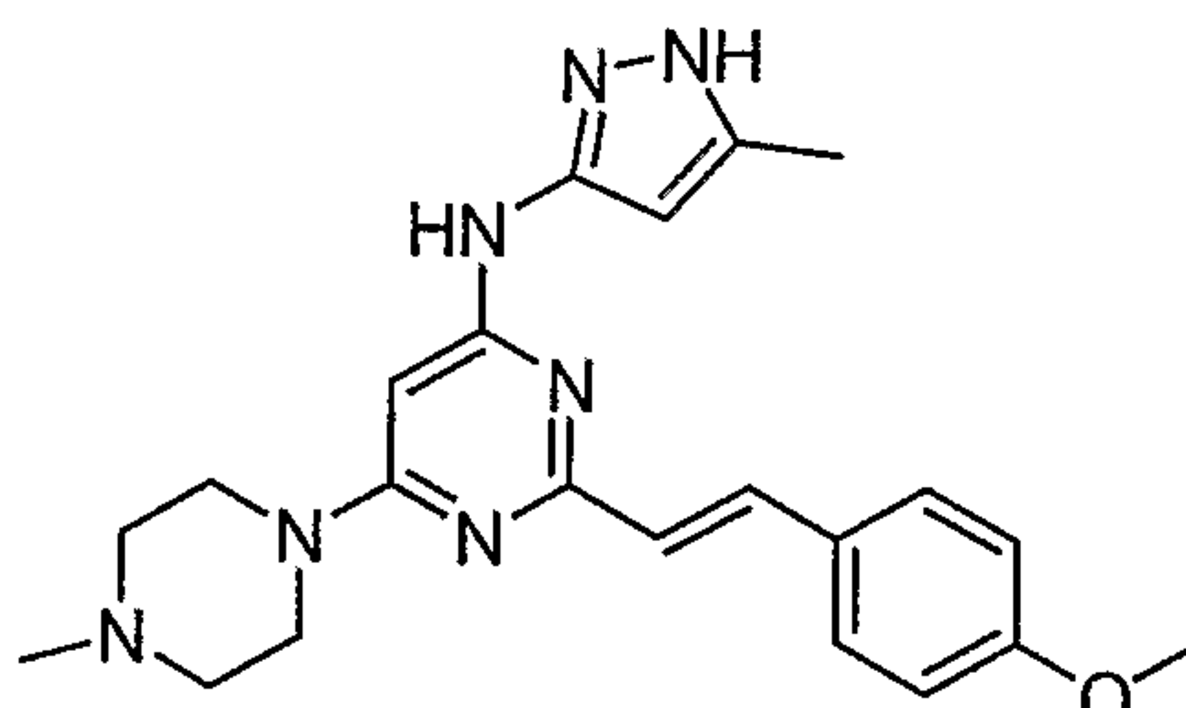
2-(4-methoxystyryl)-N-(5-methyl-1H-pyrazol-3-yl)- 6-(4-methylpiperazin-1-yl)pyrimidin-4-amine
