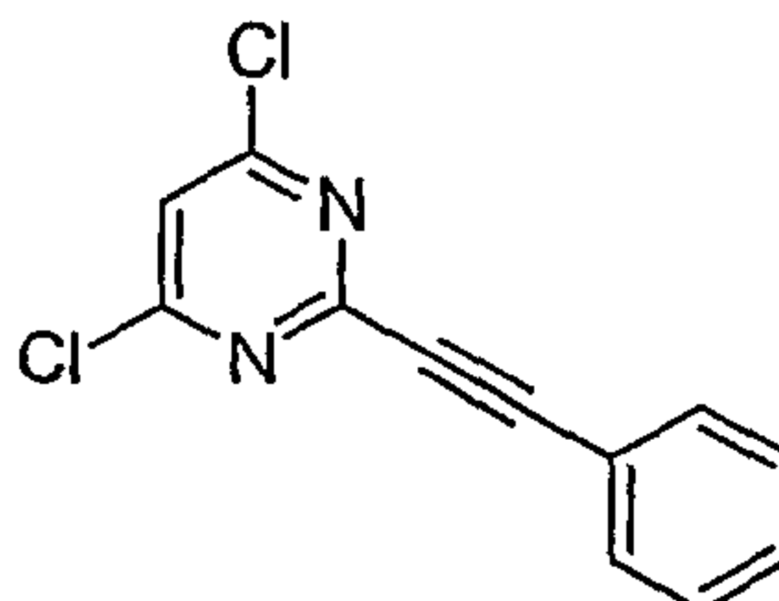
4,6-dichloro-2-(phenylethynyl)pyrimidine
