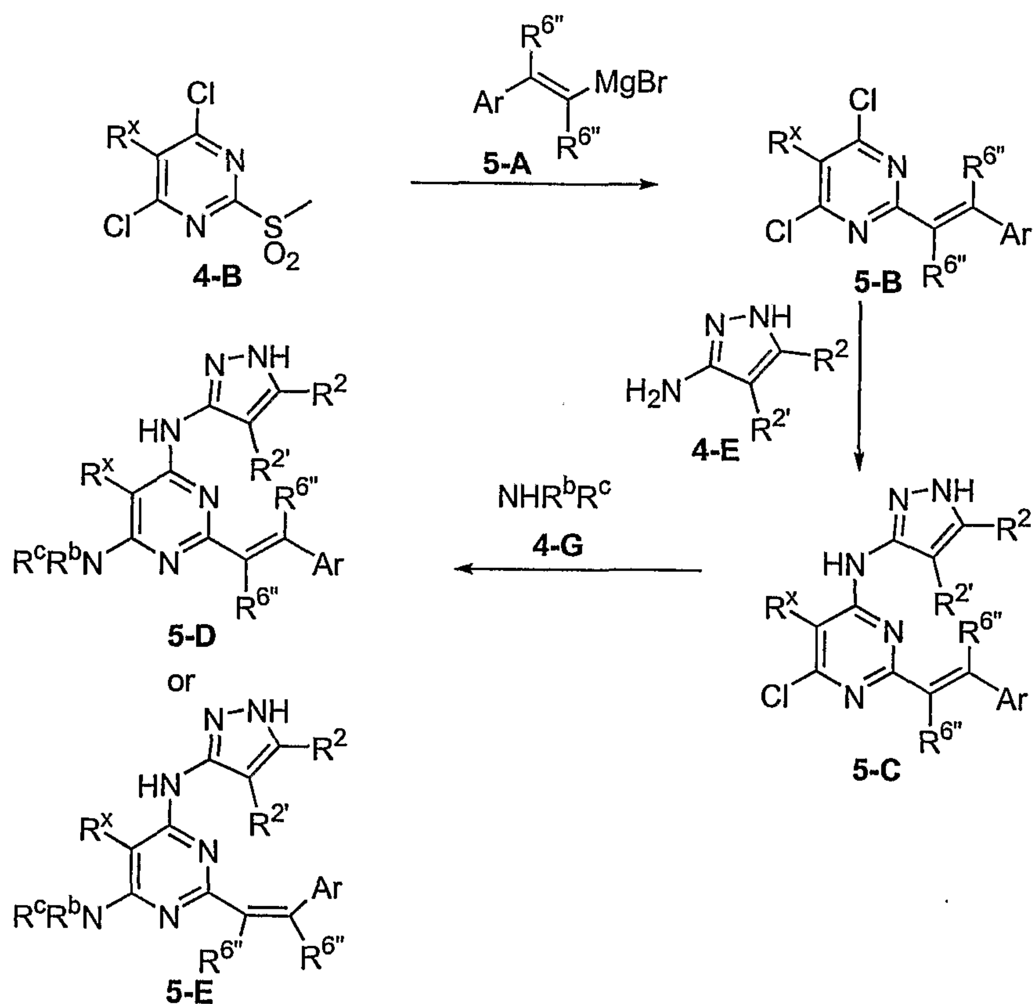
Scheme 5
