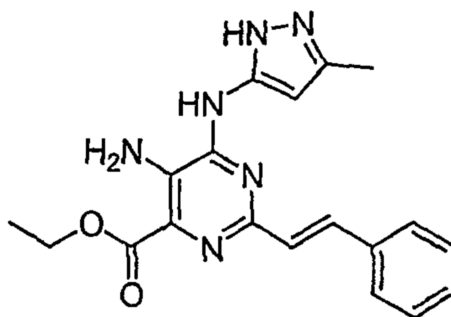
ethyl 5-amino-6-[(3-methyl-1H-pyrazol-5-yl)amino]-2-[(E)-2-phenylvinyl]pyrimidine-4-carboxylate
