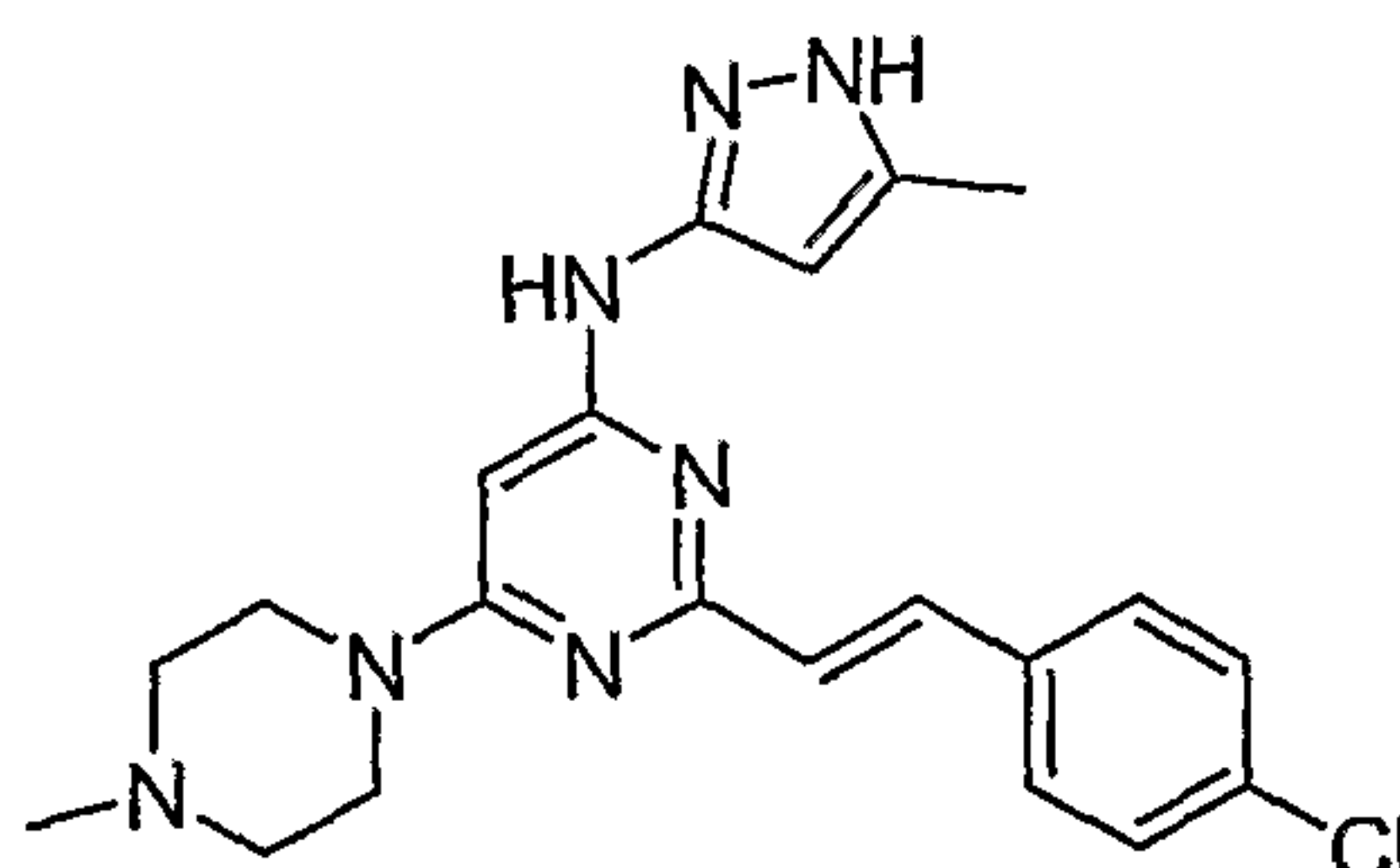
2-(4-chlorostyryl)-N-(5-methyl-1H-pyrazol-3-yl)-6-(4-methylpiperazin-1-yl)pyrimidin-4-amine
