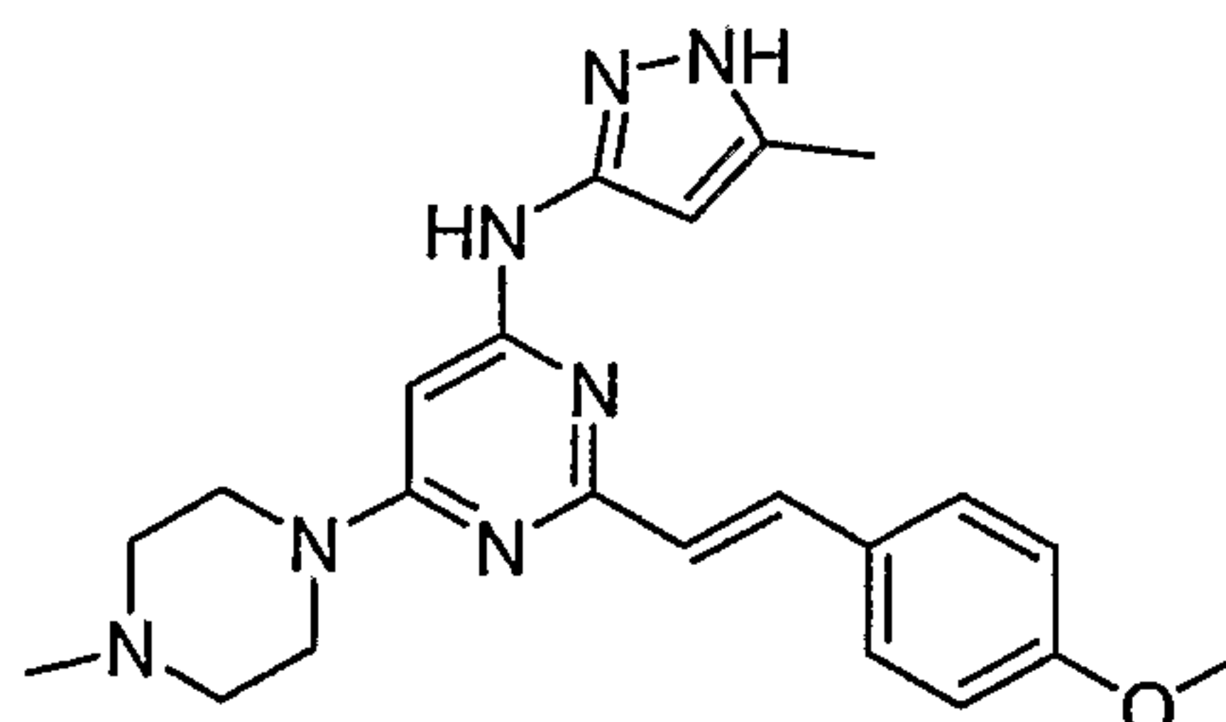
2-(4-methoxystyryl)-N-(5-methyl-1H-pyrazol-3-yl)- 6-(4-methylpiperazin-1-yl)pyrimidin-4-amine
