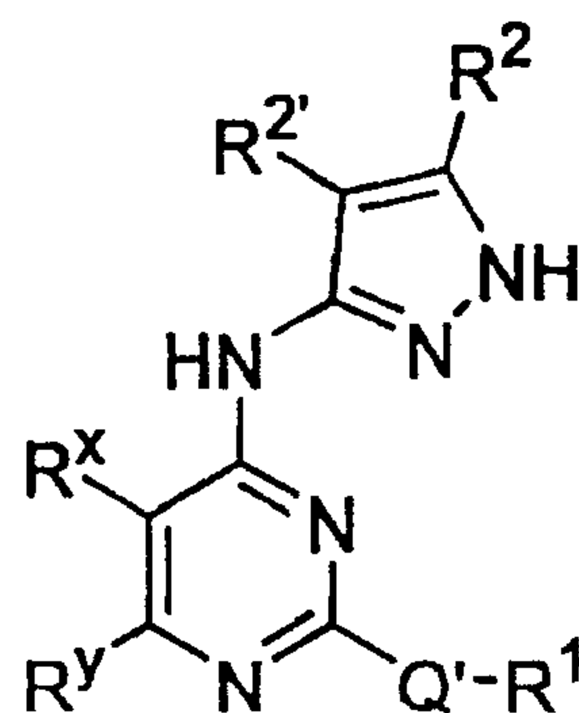
Formula I
