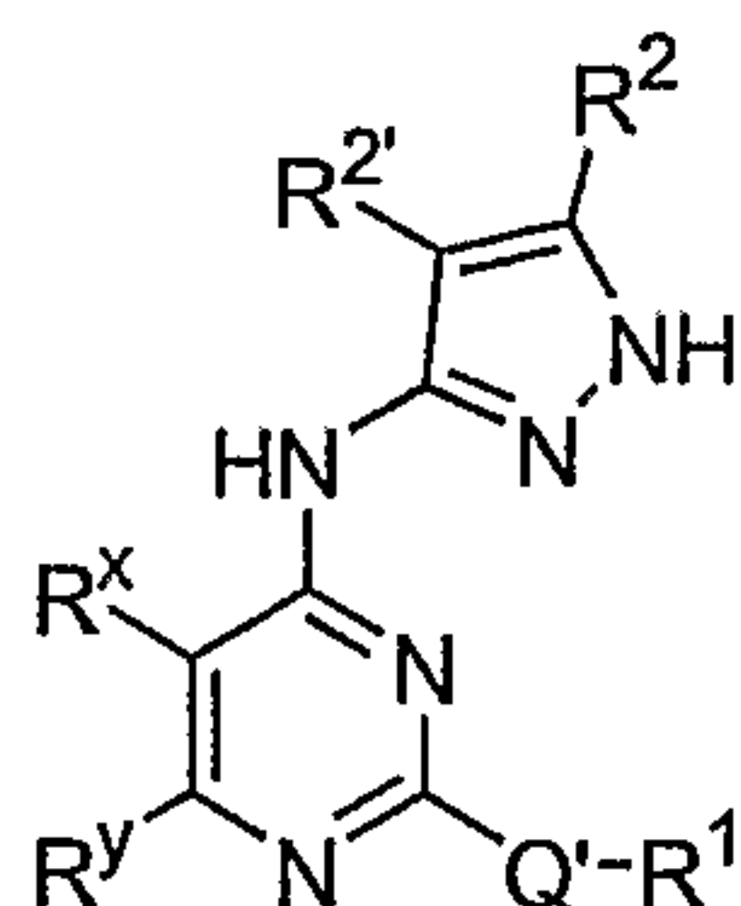
Formula I
