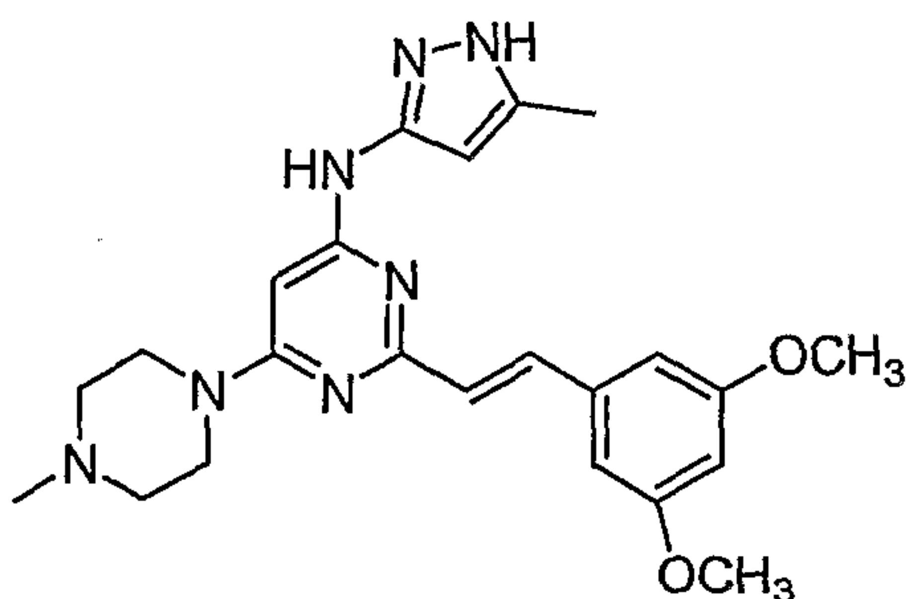
2-(3,5-dimethoxystyryl)-N-(5-methyl-1H-pyrazol-3-yl)- 6-(4-methylpiperazin-1-yl)pyrimidin-4-amine
