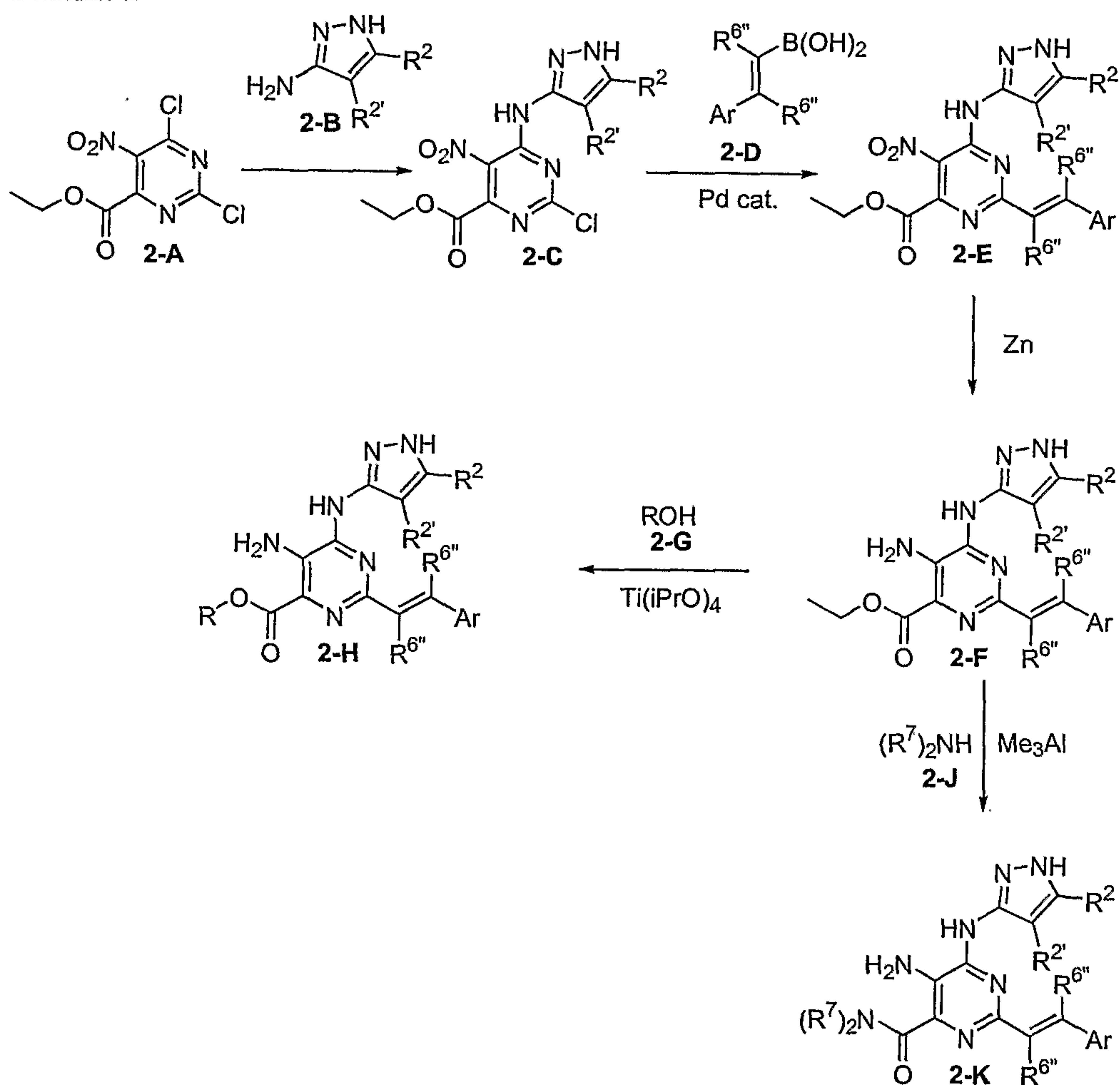
Scheme 2
