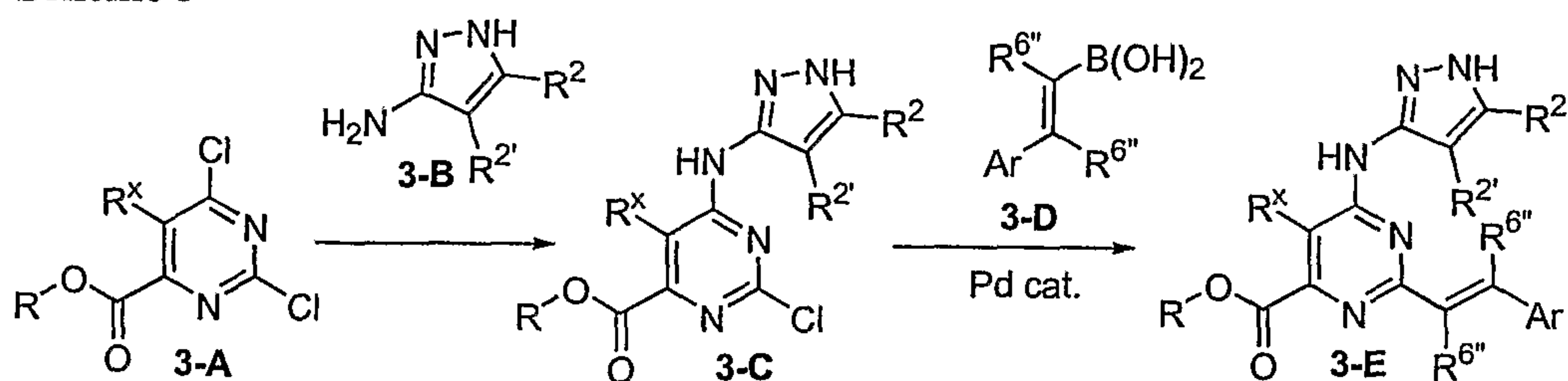
Scheme 3
