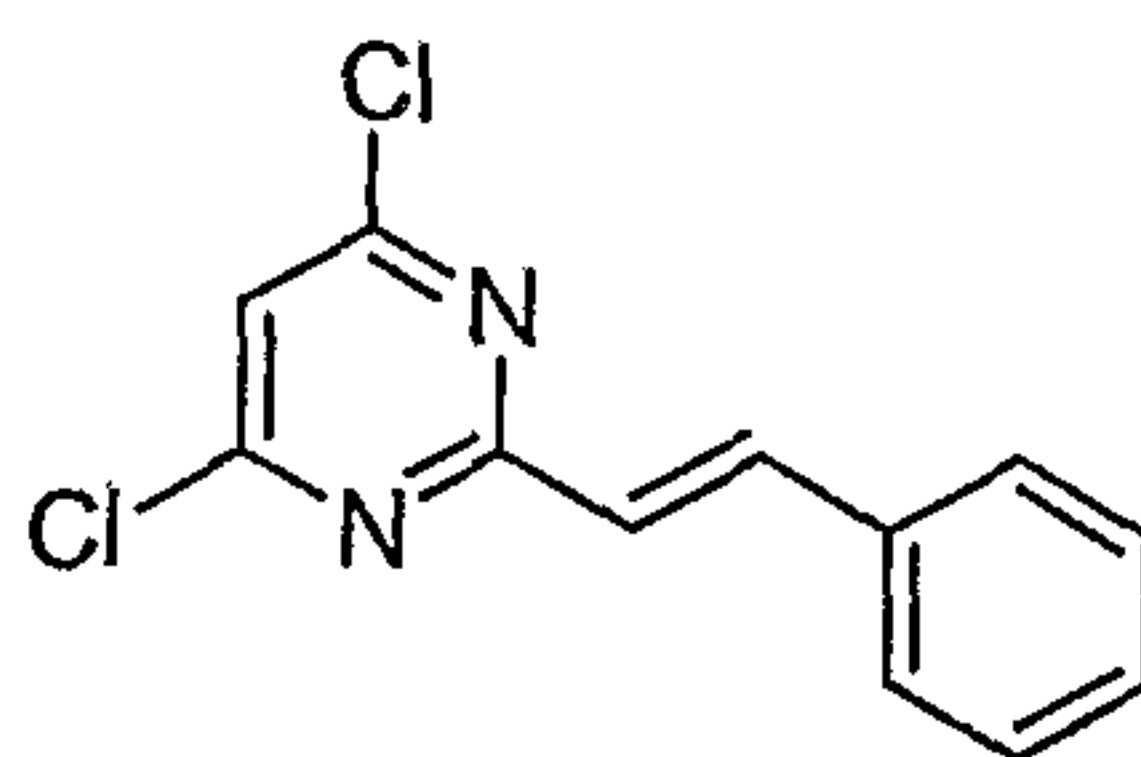
4,6-dichloro-2-[(E)-2-phenylvinyl]pyrimidine
