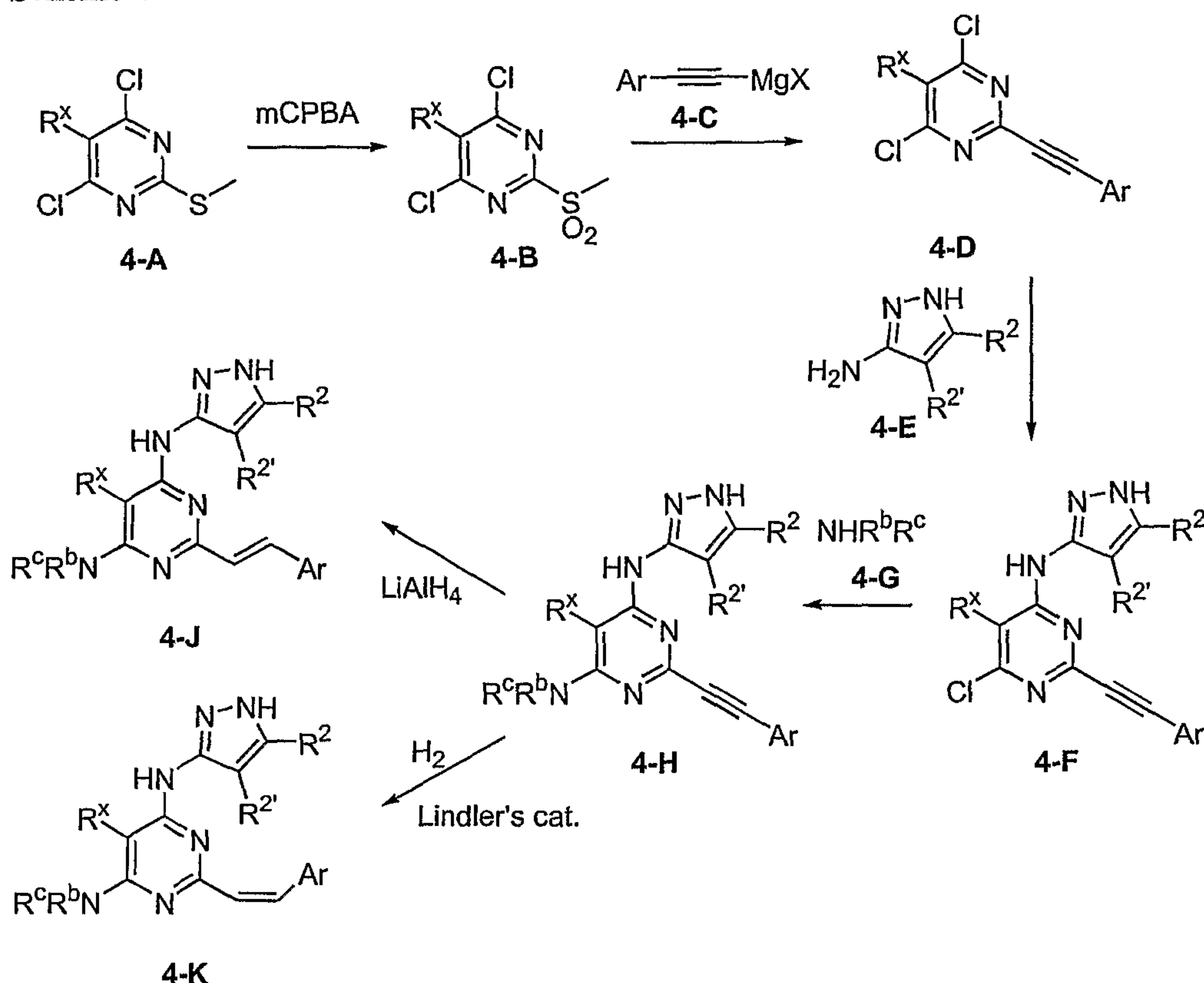
Scheme 4
