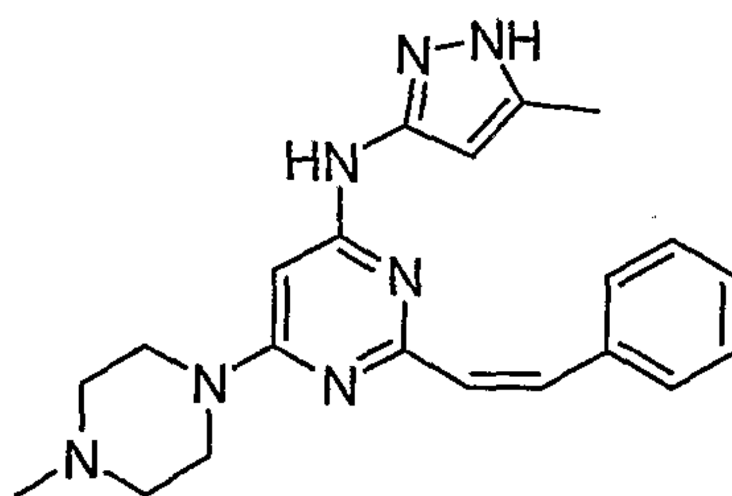
6-(4-methylpiperazin-1-yl)-N-(3-methyl-1H-pyrazol-5-yl)-2-[(Z)-2-phenylvinyl]pyrimidin-4-amine
