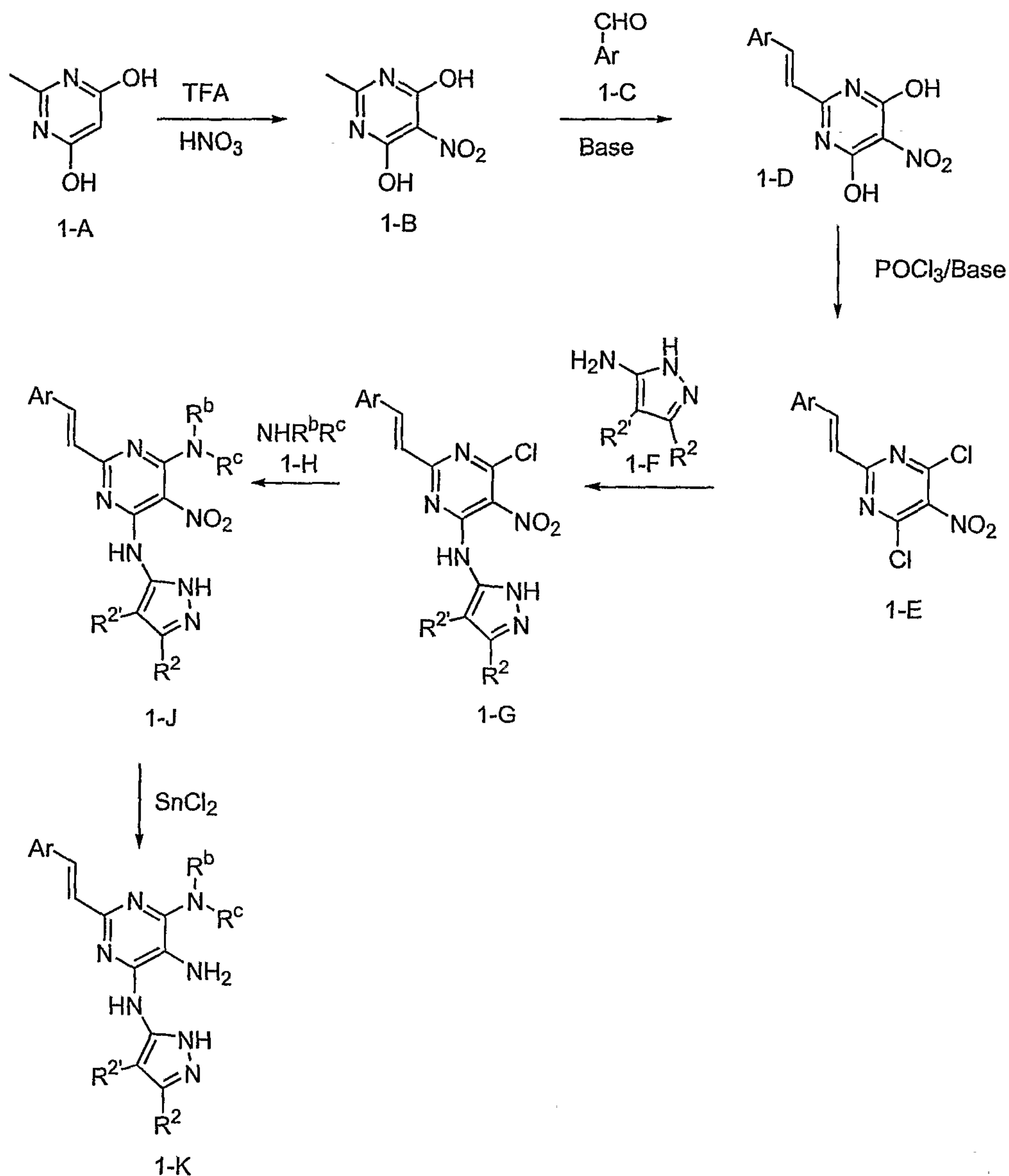
Scheme 1
