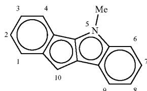
5-methylindeno[1,2-b]indolyl
