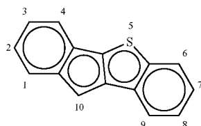
indeno[1,2-b][1]benzothiienyl
