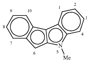
5-methylindeno[2,1-b]indolyl
