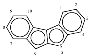
indeno[2,1-b][1]benzothiienyl
