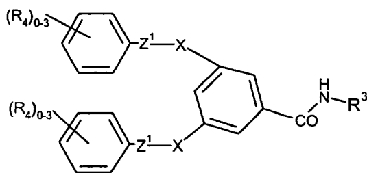
Formula (II)
