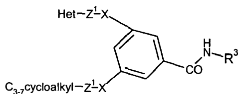
Formula (IIg)
