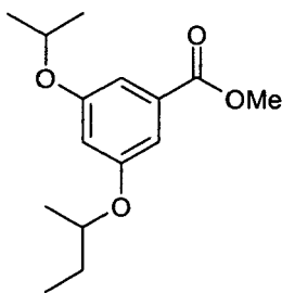
Compound (b)
