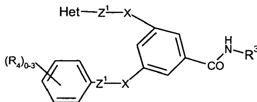
Formula (IIa)
