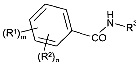
Formula (Ic)
