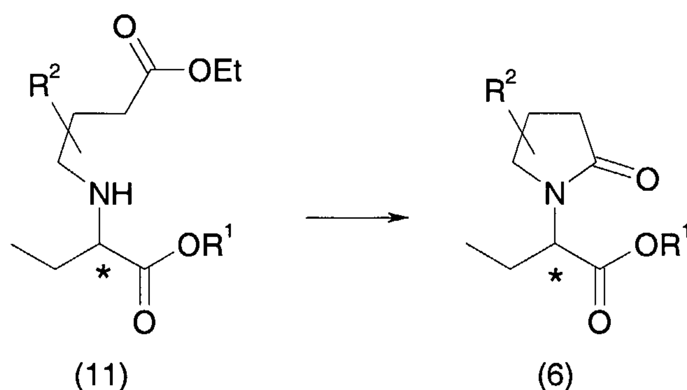
Scheme 4.
