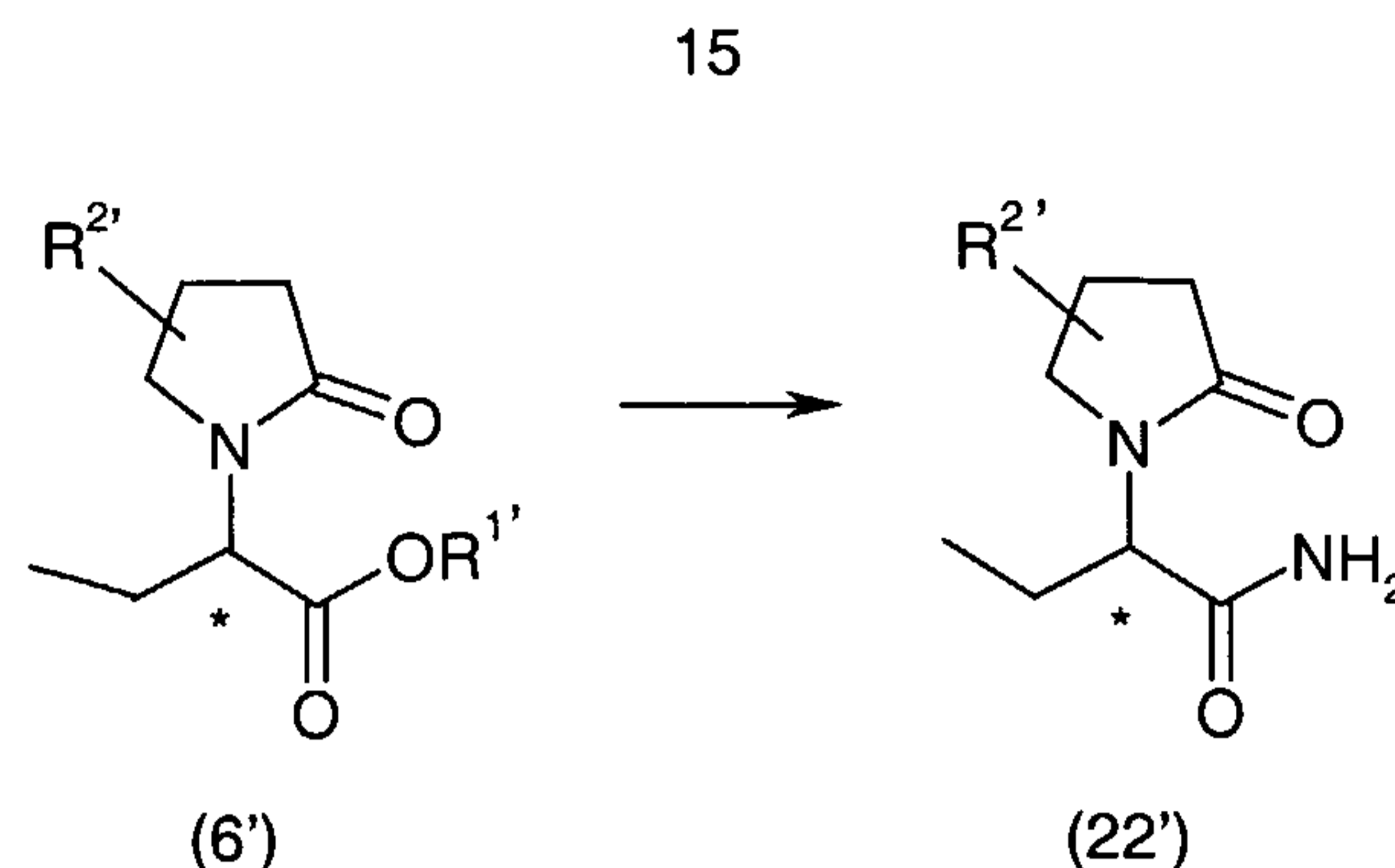
Scheme 8.
