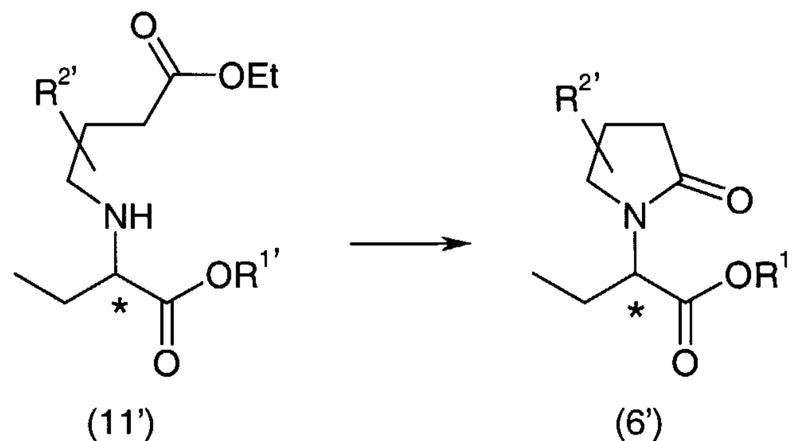
Scheme 4'.
