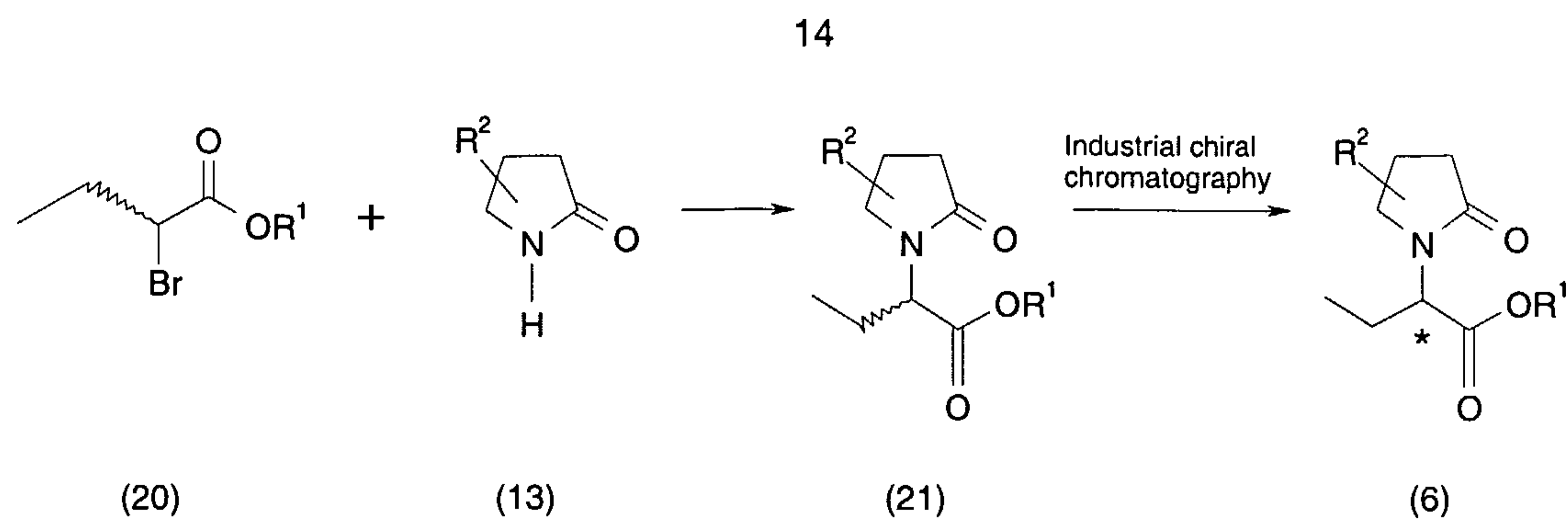
Scheme 7.
