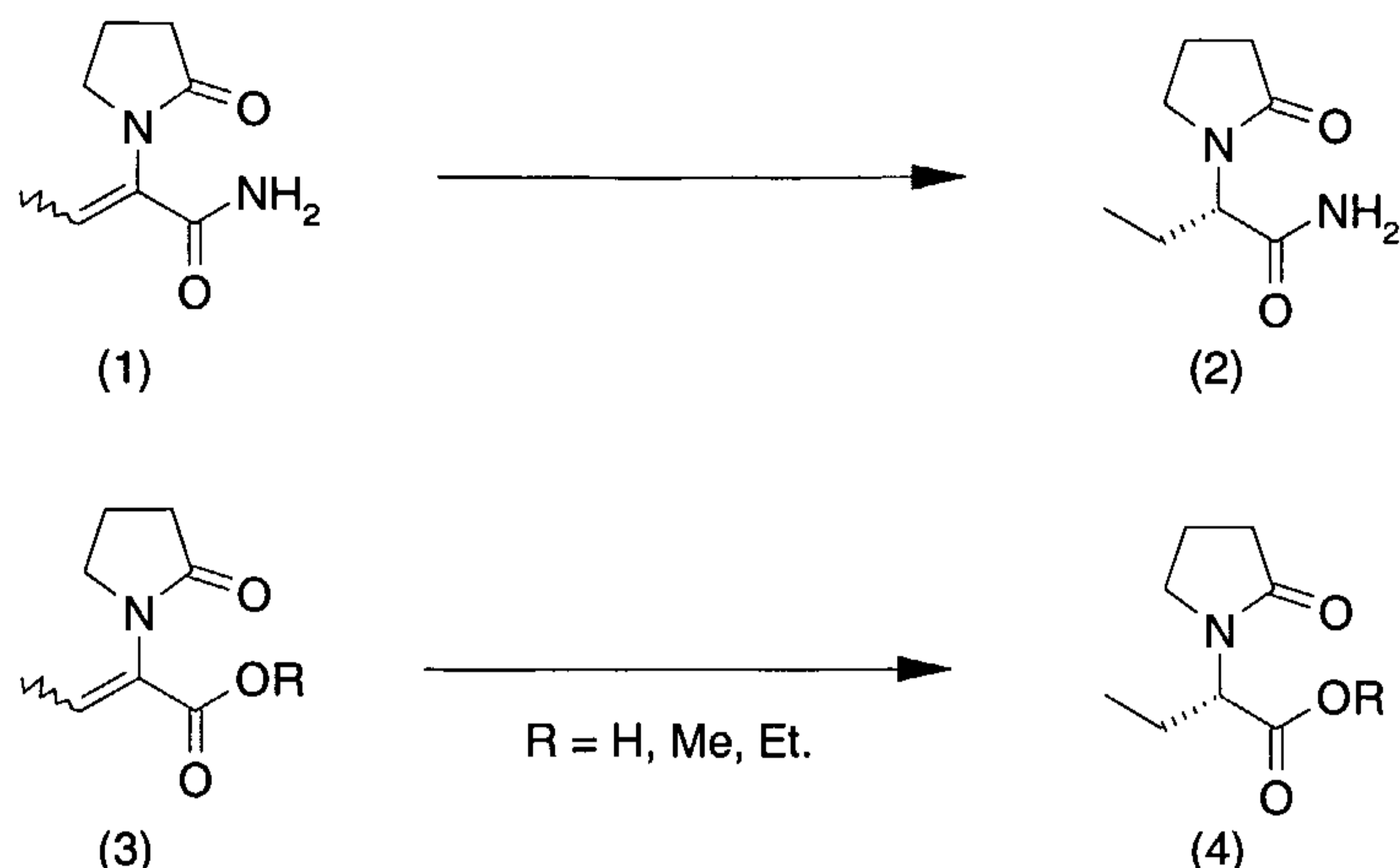
Scheme 1.
