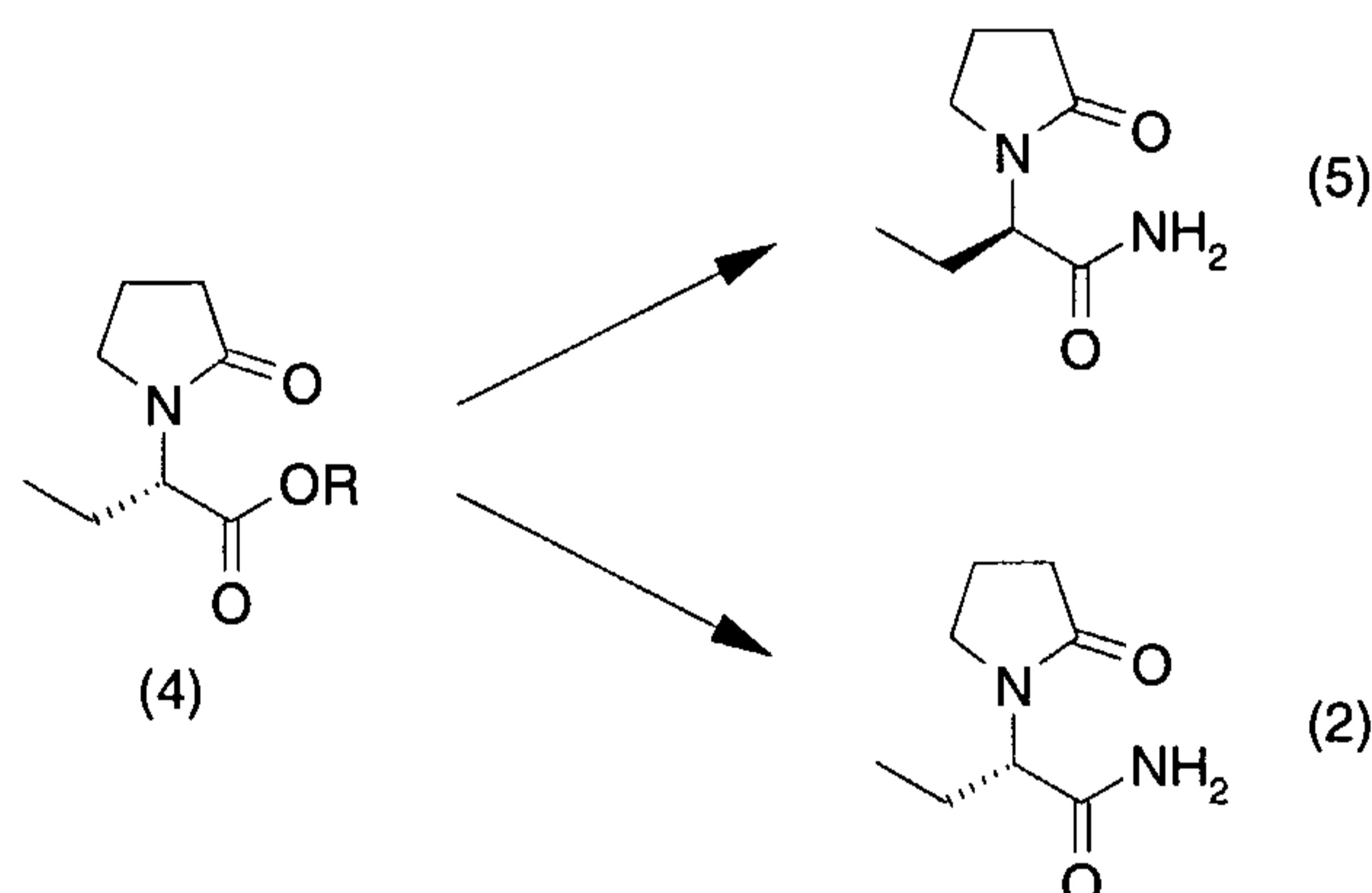
Scheme 2.
