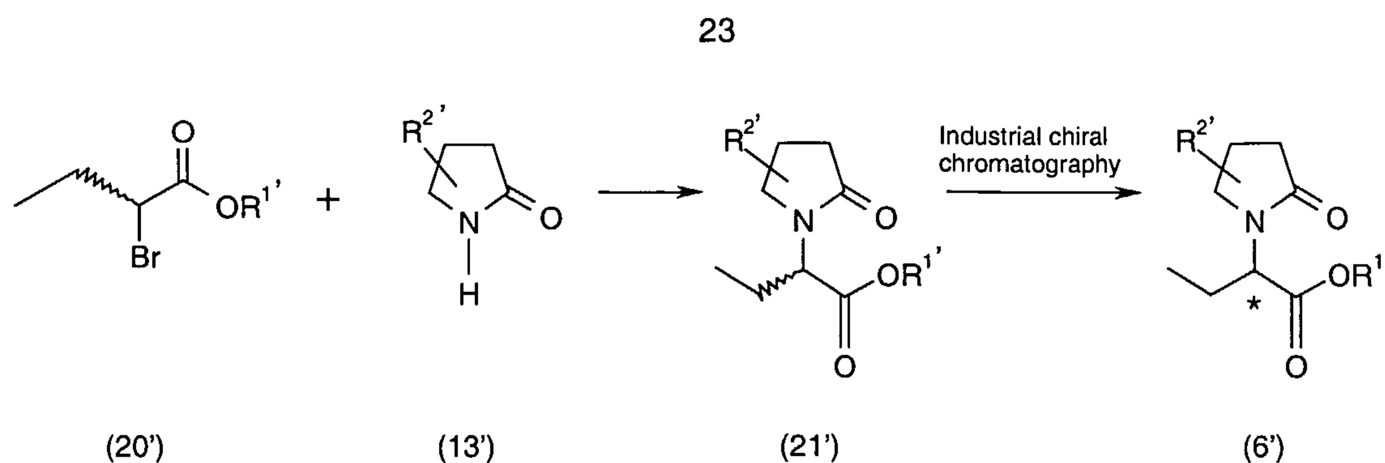
Scheme 7'.
