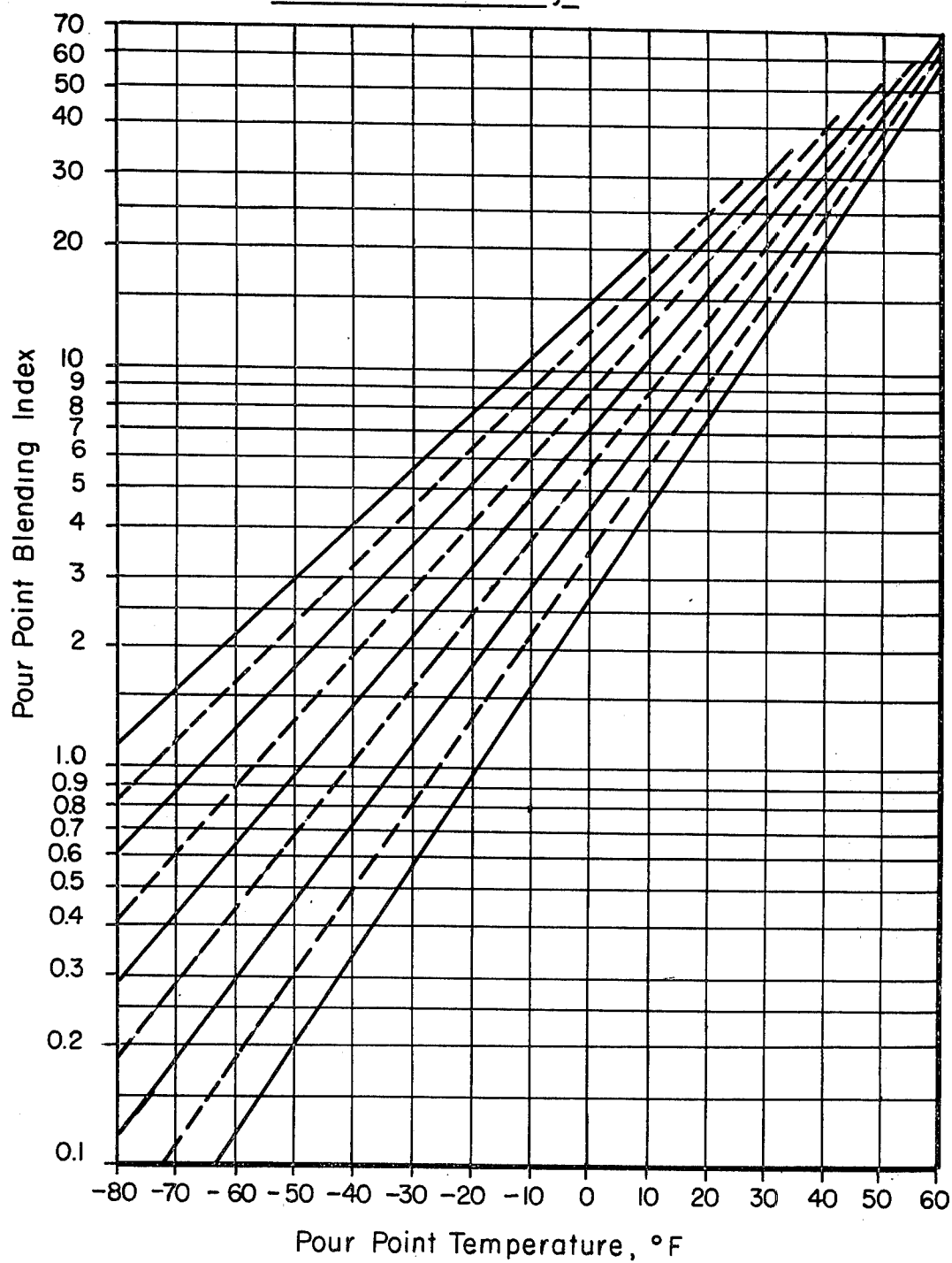
FIGURE 3 POUR POINT BLENDING CHART (Distillate Blends Only)
