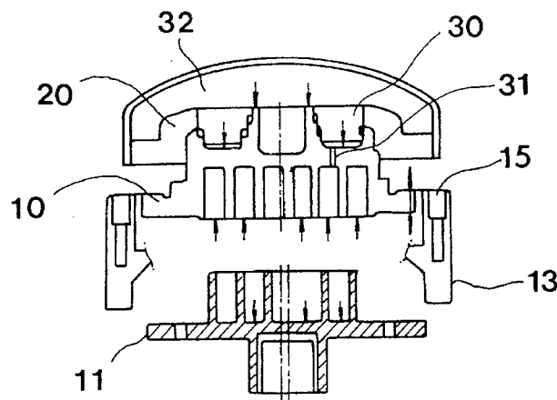
FIG. 6 PRIOR ART
