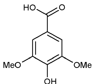
4-Hydroxy-3,5-dimethoxybenzoic acid (syringic acid)
