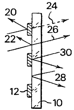
FIG 1c (Prior Art)
