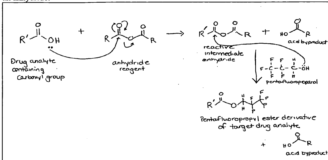
Figure 3: Esterification of a carboxyl group using pentafluoropropanol in the presence of an anhydride.
