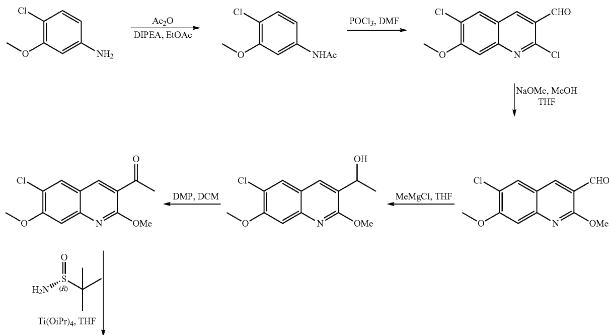
Scheme 3
