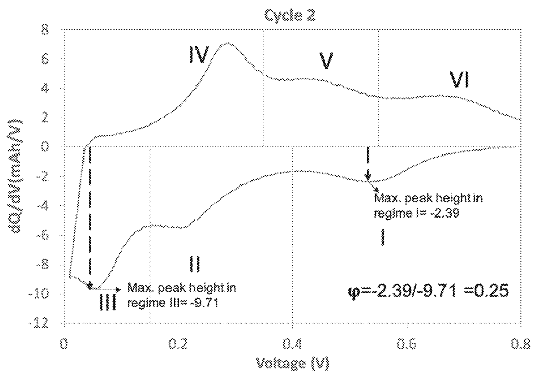
Figure 5. Example of calculation of \phi for Silicon-Carbon Composite 3.
