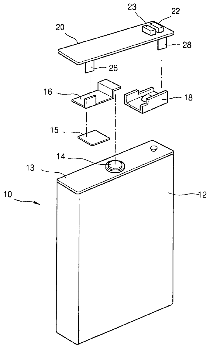
FIG. 2 (PRIOR ART)
