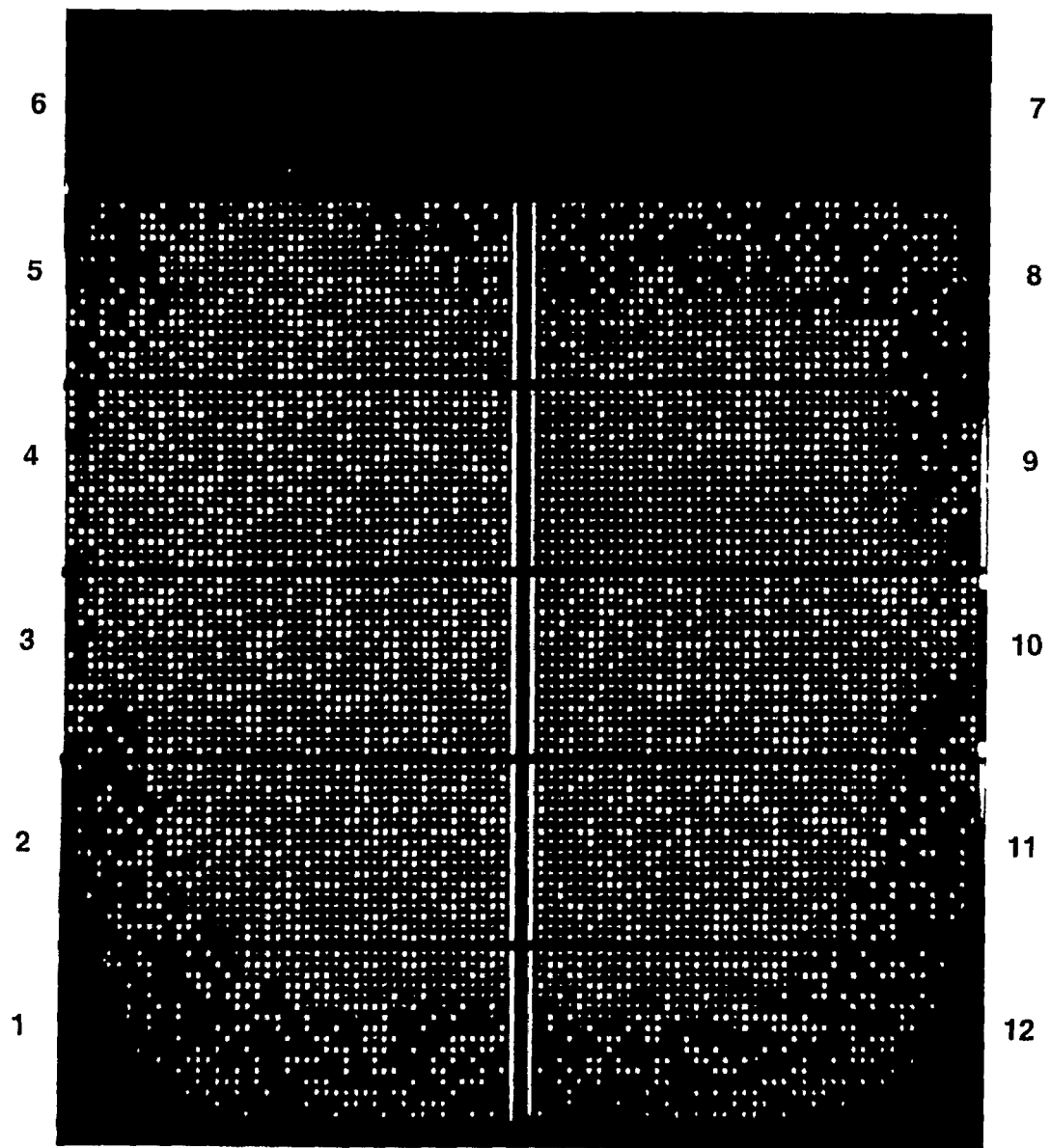
Chr21 FAM
