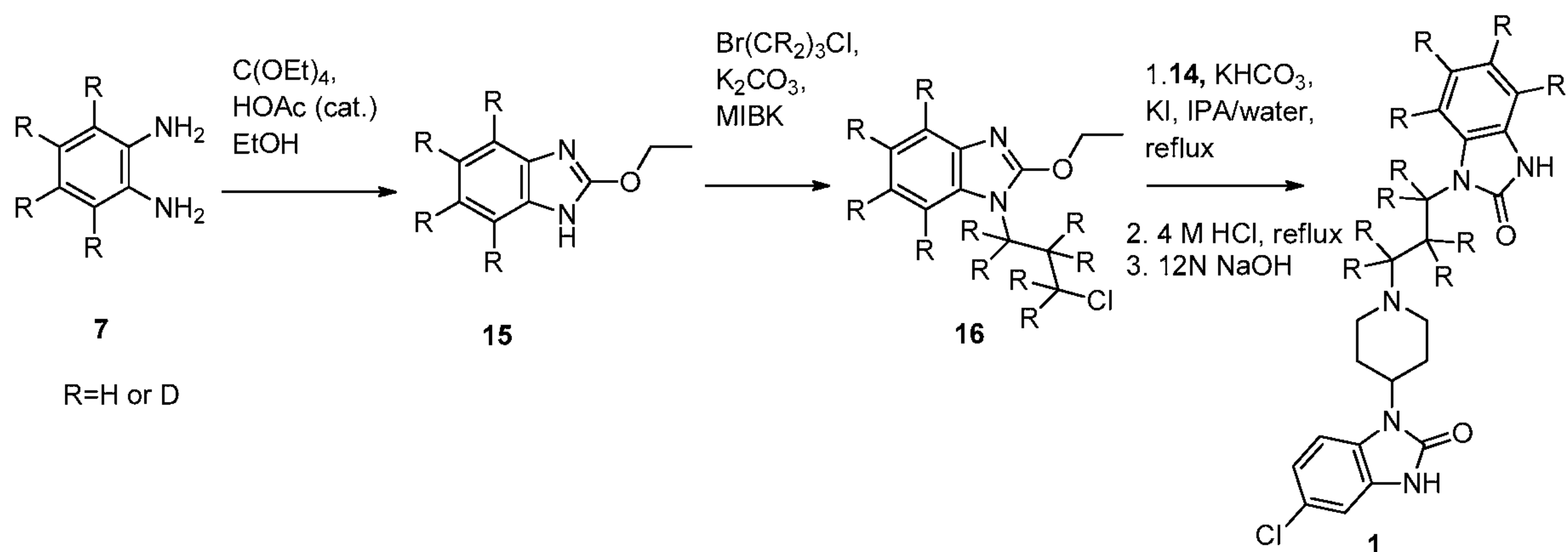
Scheme 2 Synthesis of Deuterated Domperidone
