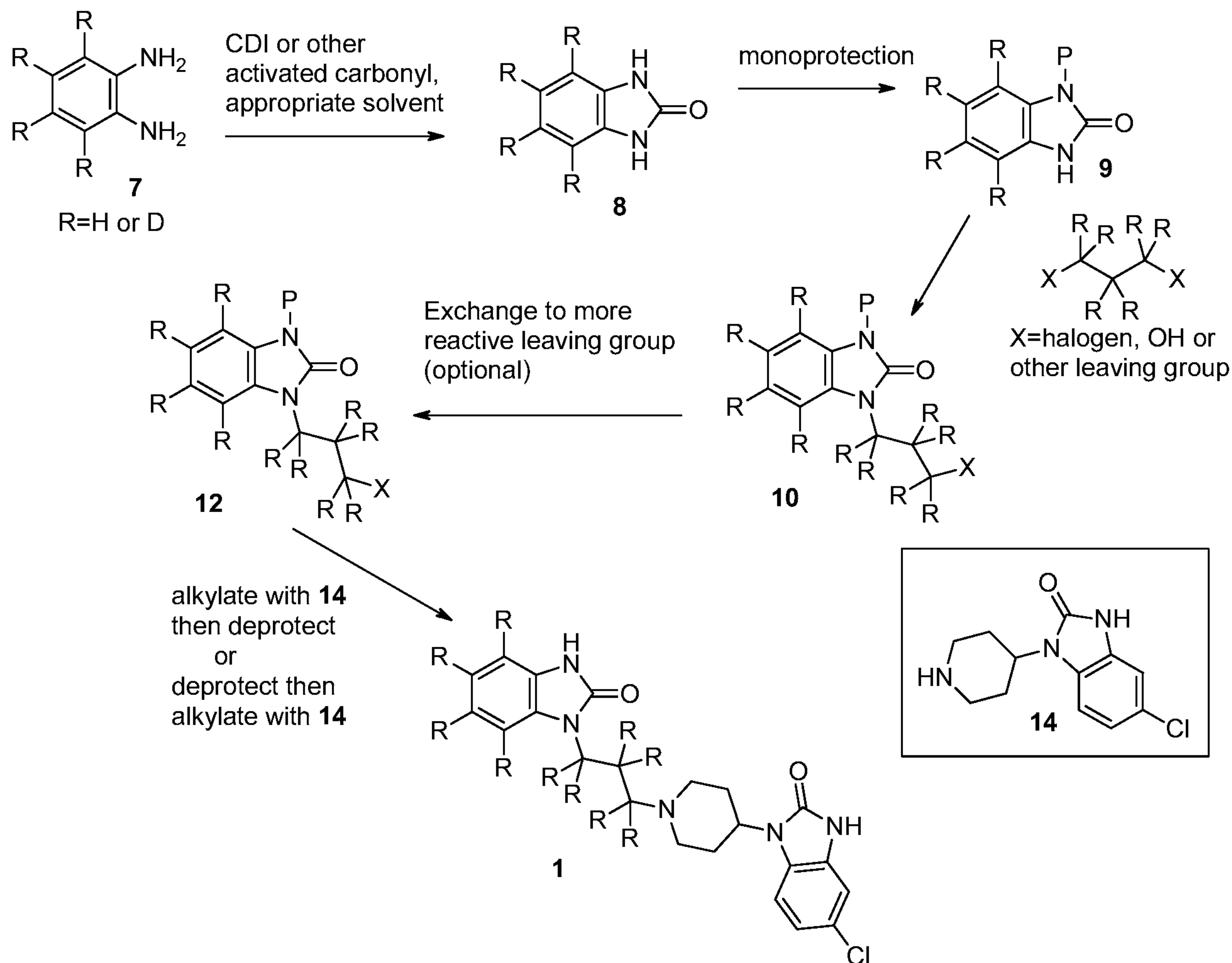
Scheme 1: General Synthesis of Deuterated Domperidone
