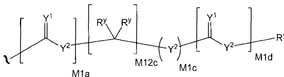
Formula IVb
