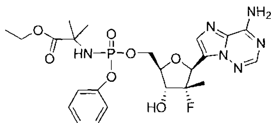
Compound PD-A-8h
