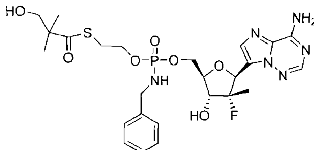
Compound PD-F-8w
