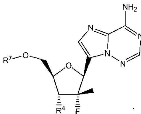
Formula VI
